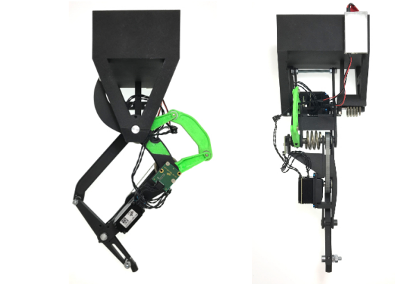
Fig. 1: Front and side view of the proposed articulated soft robotic leg prototype. We embed during the design phase a SLIP-like behavior when the leg is close to the vertical configuration. This is done by selecting suitable physical parameters in order to embed a vertical strict mode in the dynamics. As a result, the leg can efficiently jump in place exploiting its natural dynamics.
