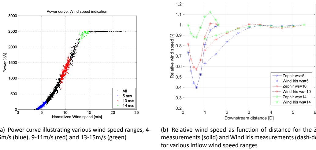
Figure 9: Wake recovery in the 'undisturbed' sector [53]
