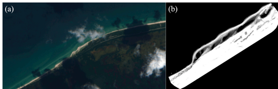
Fig. 12. (a) Satellite images from Sentinel 2 (October 14, 2021) showing formation of a longshore sand wave at Punta Piedra (northwestern Yucatan coast) consistent with the nearshore bar attachment model by Stewart and Davidson-Arnott (1988). (b) A digital terrain model from this study area obtained in December 2022 showing the sand spits and runnels.
