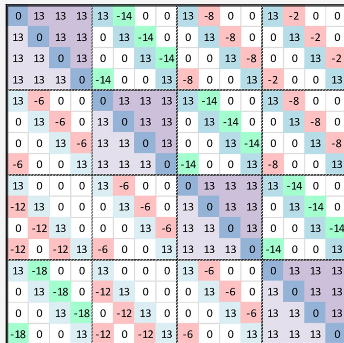
Fig 7. Q-matrix for de novo example.
