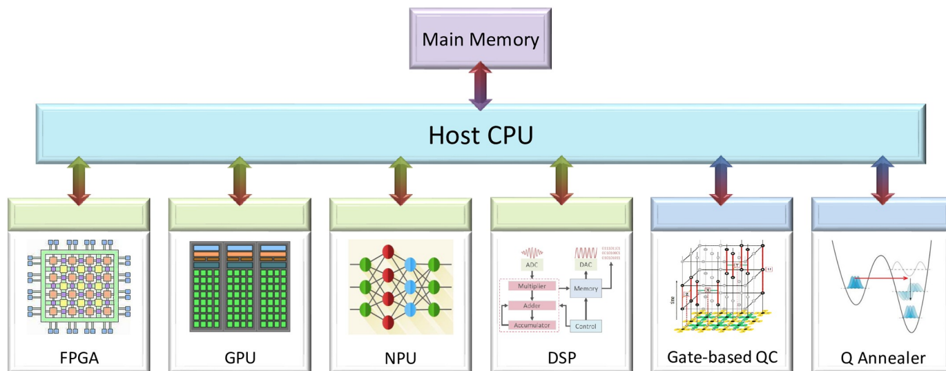
Fig 1. The accelerator model of computing.
