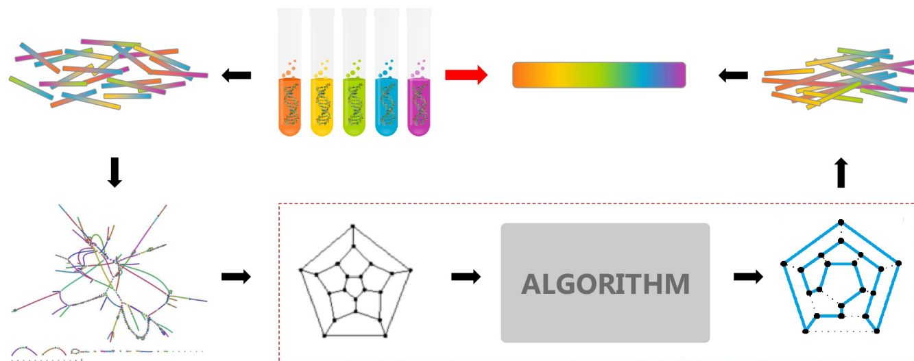
Fig 2. Overlap-layout-consensus genome assembly algorithm.
