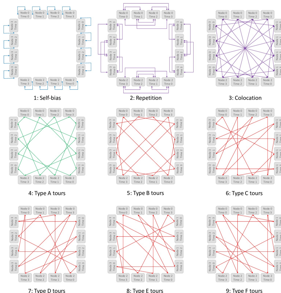
Fig 6. QUBO interactions.
