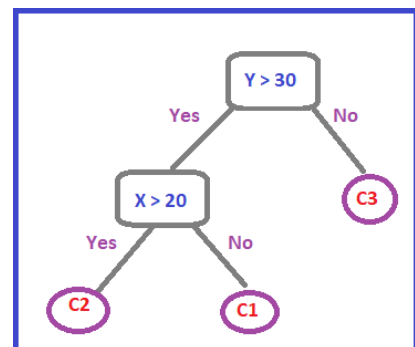
Figure 3. Corresponding decision tree for the dataset depicted in Figure 2
