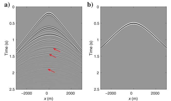
Figure 2. (a) The modeled reflection response with source and receivers at the acquisition surface. The red arrows indicate the internal multiple reflections. (b) The modeled first arrival of the downgoing Green's function with source at the focal point in the subsurface and receivers at the acquisition surface.
