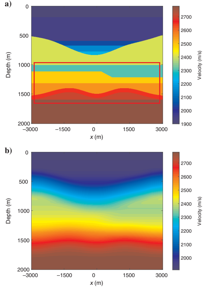
Figure 1. (a) Velocity model that will be used to model the reflection response, and the red box gives the target zone that will be imaged. (b) The smoothed velocity model that will be used to model the first arrival of the downgoing Green's function.
