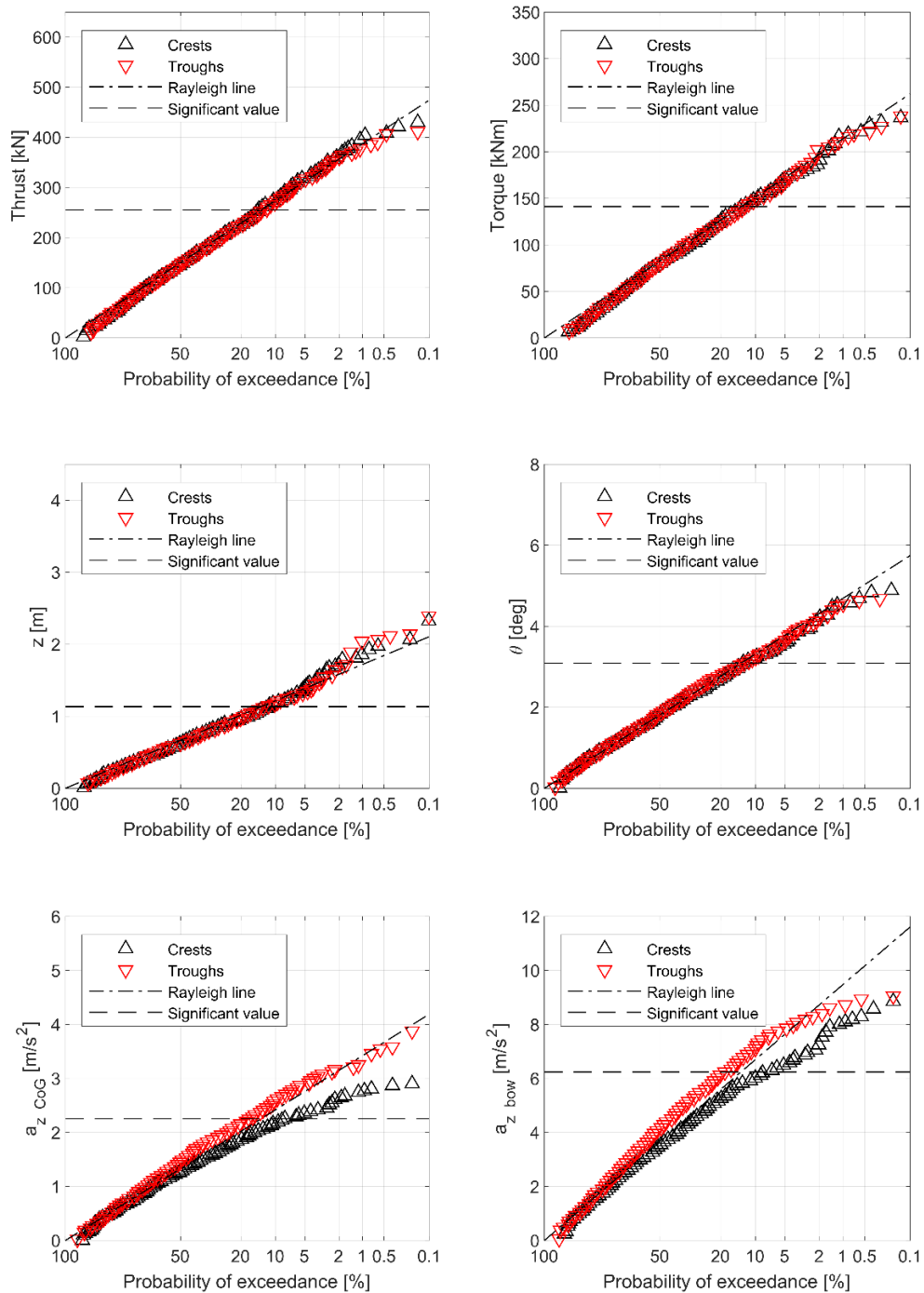
Figure 14: Distribution plots of the FCS frigate
