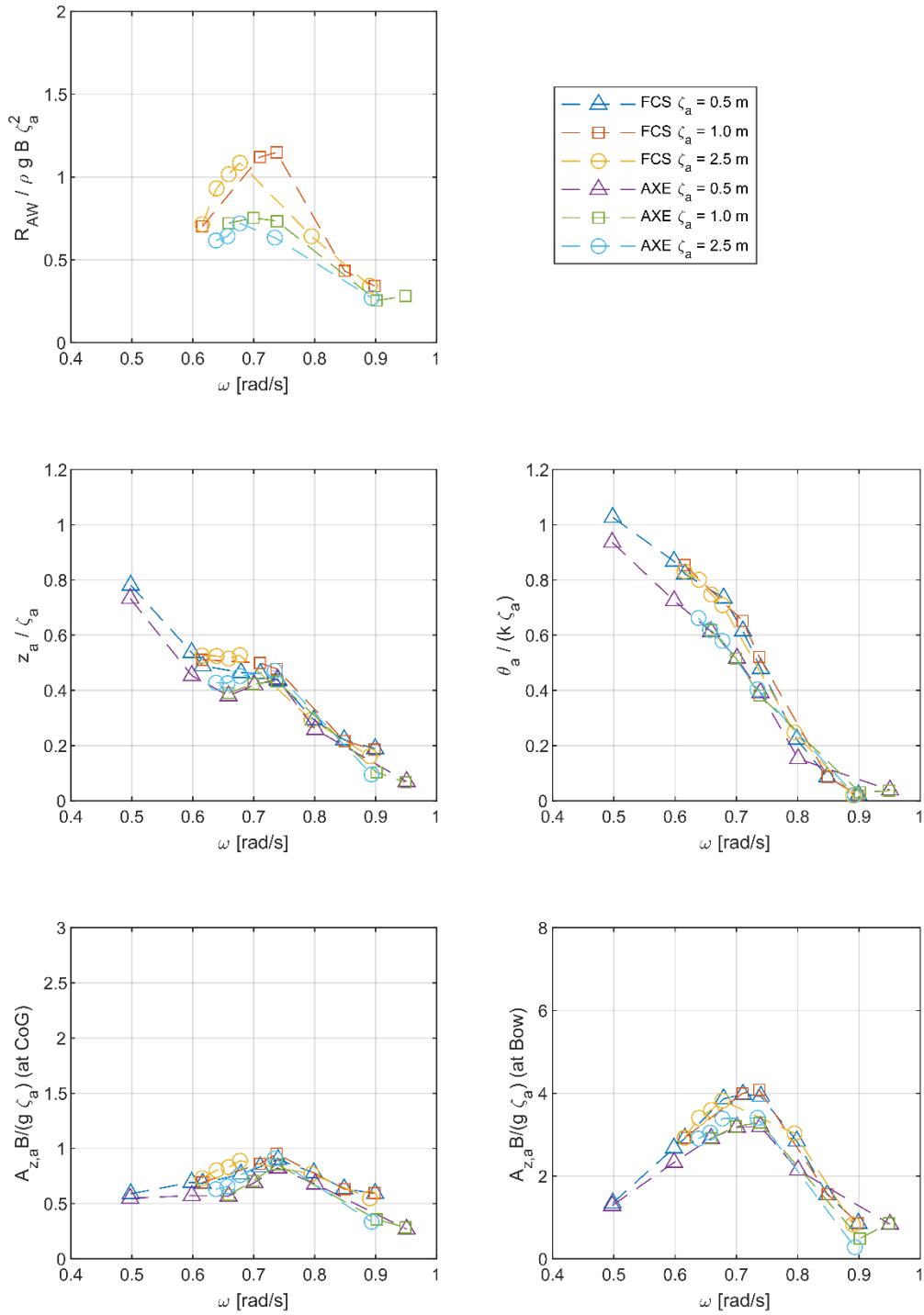
Figure 7: Comparison of the ship response between the FSC and AXE frigates at a forward speed of 15 knots
