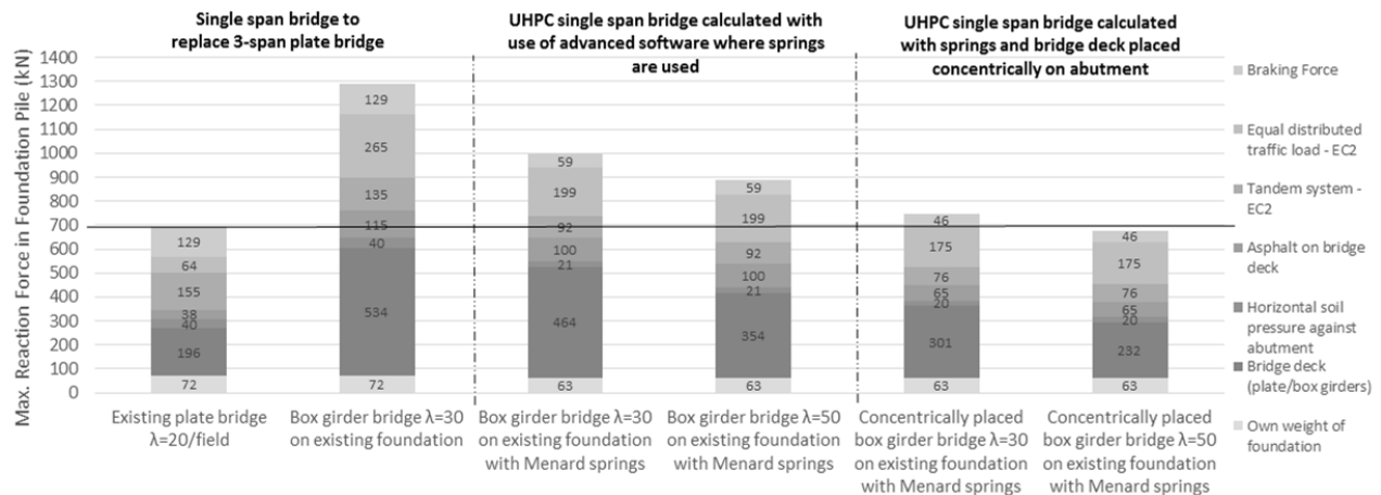
Fig. 12. Maximum reaction force in existing foundation piles obtained by different calculation methods.
