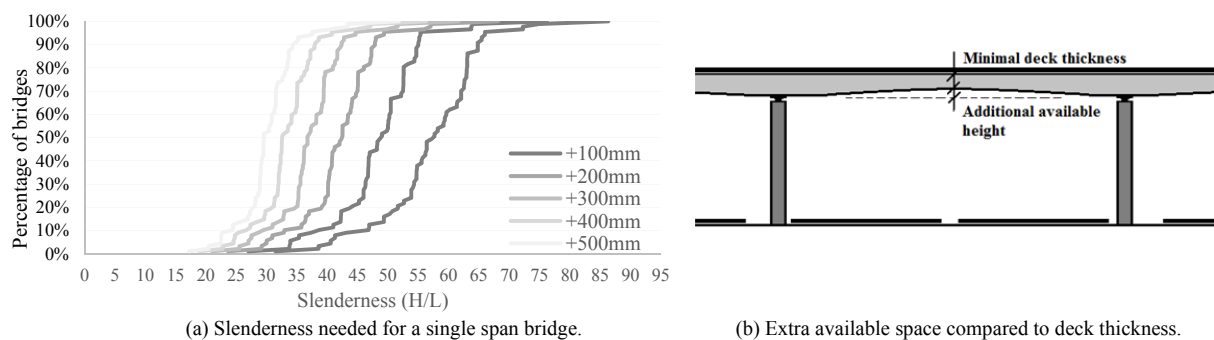
Fig. 5. Identification of slenderness needed to replace existing three span plate bridges.
