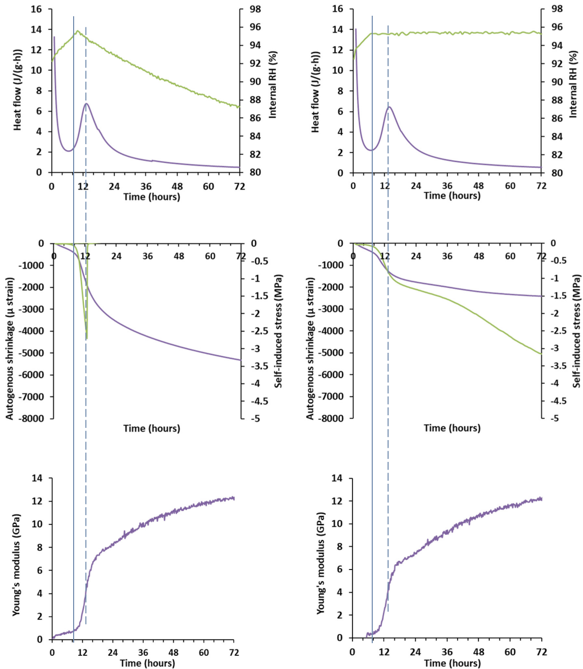
Fig. 12. Heat flow plotted together with internal RH, autogenous shrinkage, self-induced stress and Young's modulus of (left) AAS0.5 and (right) AAS0.552SAP. 0 h of all the curves represents the moment of adding liquid.
