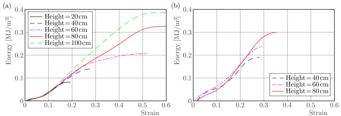
Fig. 8. Absorbed specific energy profiles of (a) low-density and (b) high-density foams impacted by an impactor with 1.3 kg weight
