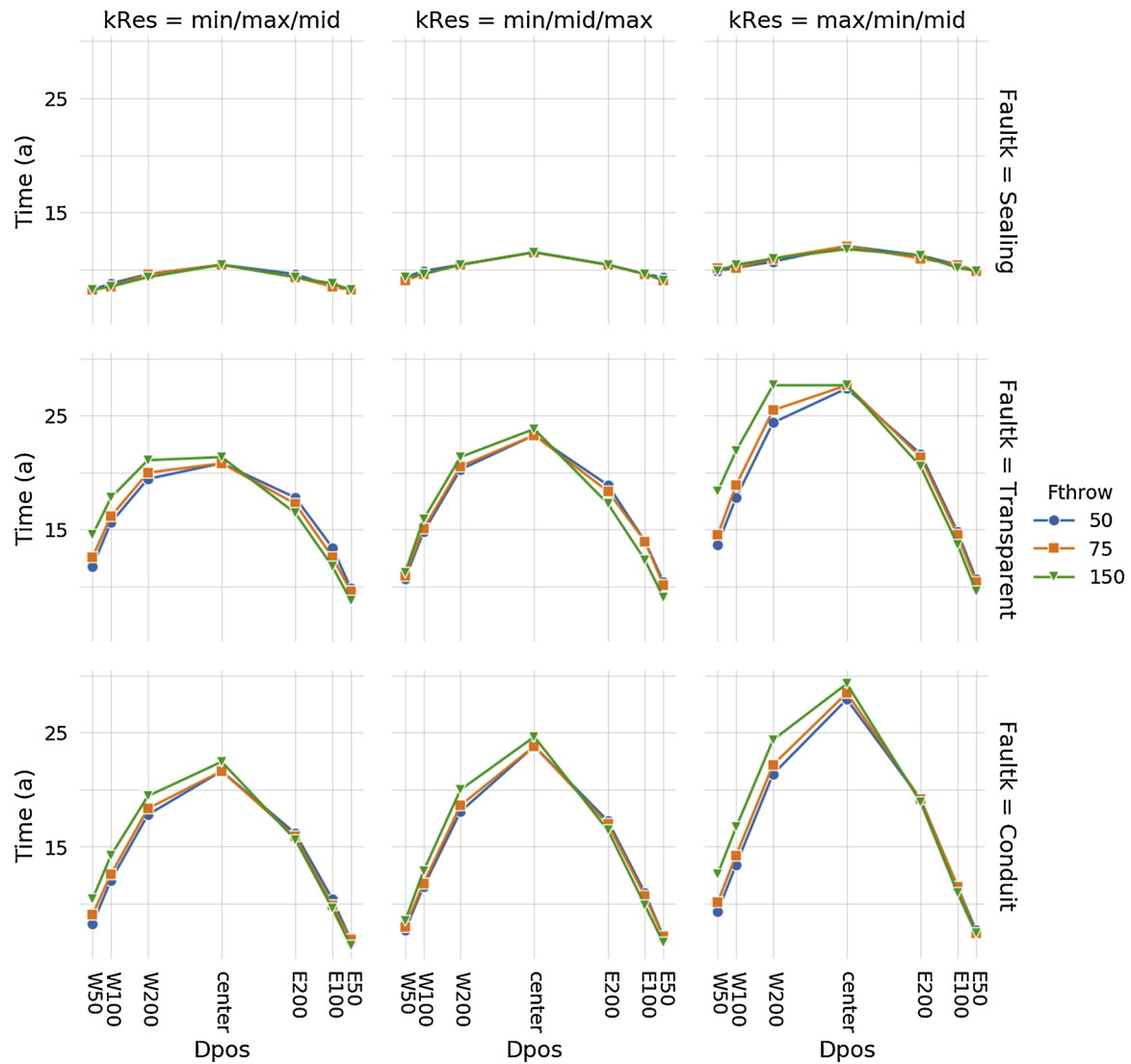
Fig. 6. Effect of fault permeability (rows), reservoir architecture (columns), doublet distance to fault (x axis) and fault throw (colour) on the system lifetime (y axis) for the series fault type. A well spacing of 800 m is used for all data points. The system lifetime criterion is defined in section System lifetime and NPV.
