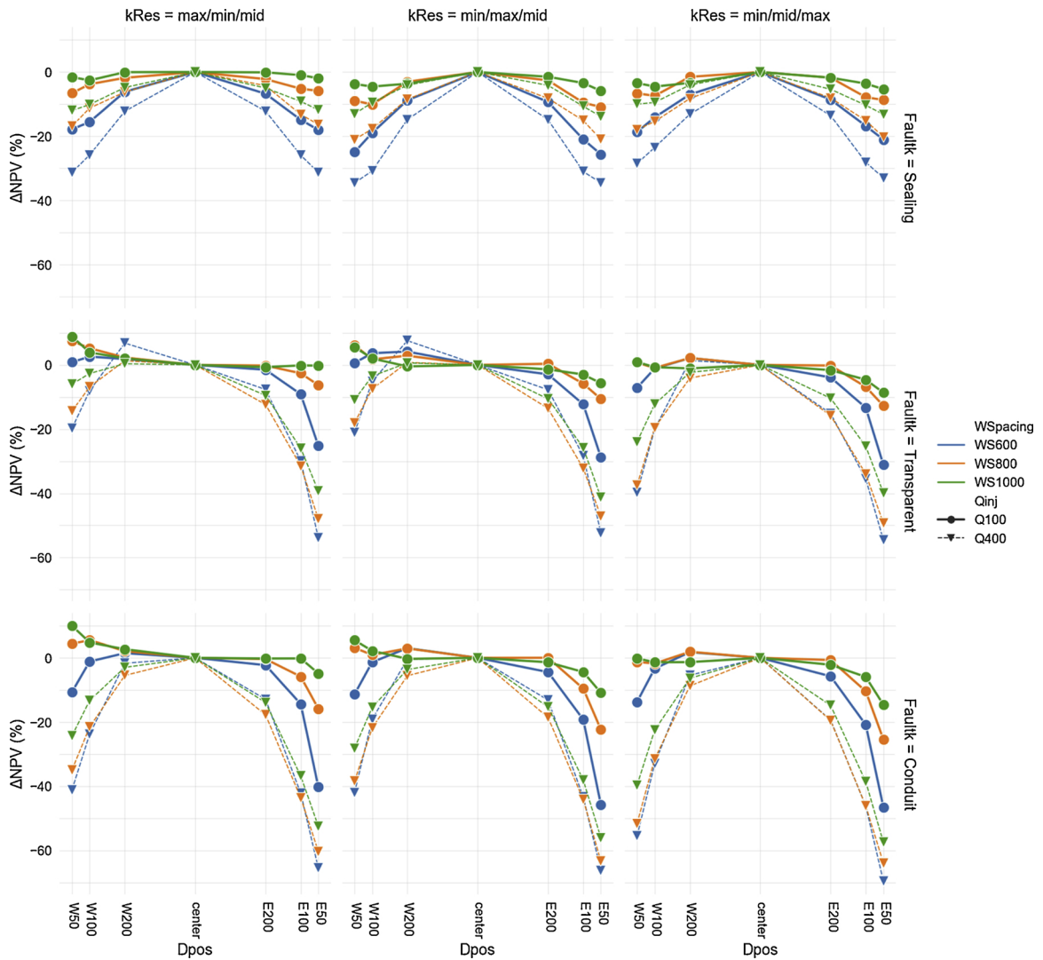
Fig. 11. Changes in NPV (%) (y axis) for different doublet positions in relation to the faults (x axis), different fault permeability (rows) and different reservoir architectures (columns) for the subset of data with a series fault type and fault throw of 150 m. The data are colour coded according to the well spacing and different flow rates are indicated by the line style.
