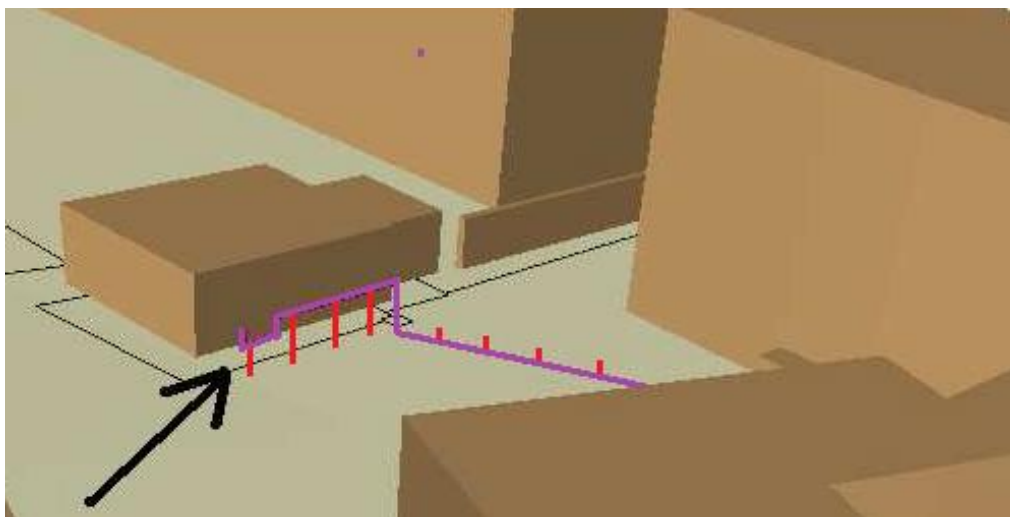
Figure 19. The pipeline (the purple line, starts above ground near arrow and is partly below ground). The black lines on the surface are the normal 2D parcel boundaries. The virtual ‘red sticks’ show vertical distance to surface, this is a clue for above/below the surface and the actual depth/height, and can be switched on/off. Source background: (Vandysheva et al. 2012)
