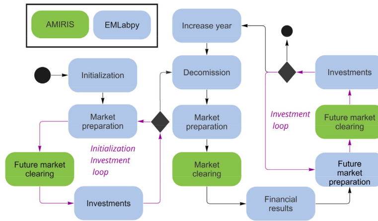
Fig. 1. Overview of the co-simulation methodology.
