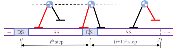
Fig. 3. Bipedal walking with support switch. The DS phase at the ending of the next ((i+1)\text{th}) step is ignored.
