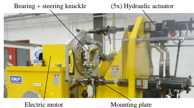
Fig. 8. The bearing test system located at our industrial partner
