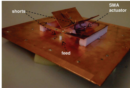
FIGURE 15: Reconfigurable square ring-patch antenna with dual-flap ground-shorted parasitic patch [31].
