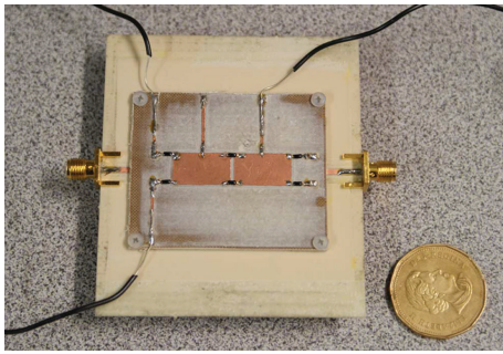
FIGURE 7: Frequency tunable differentially fed patch antenna [14].
