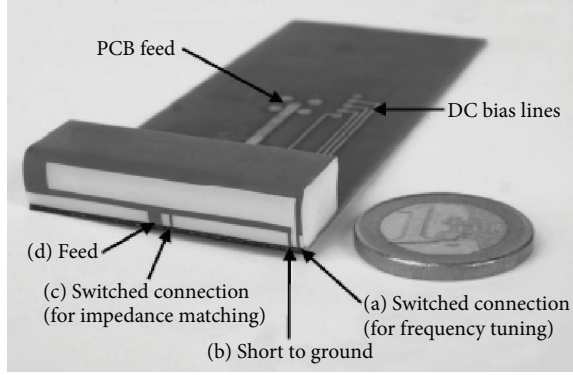
FIGURE 2: Frequency switchable PIFA antenna with MEMS [4].
