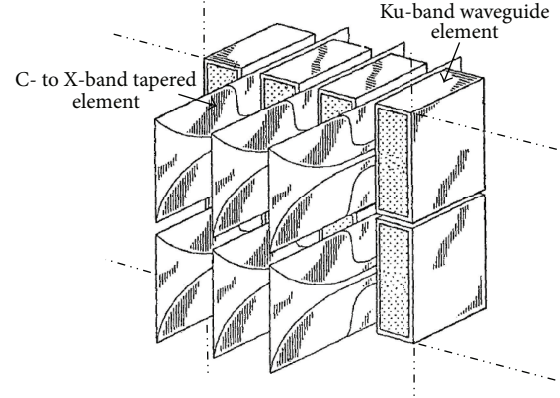
FIGURE 25: Multiband phased-array antenna with interleaved elements [62].
