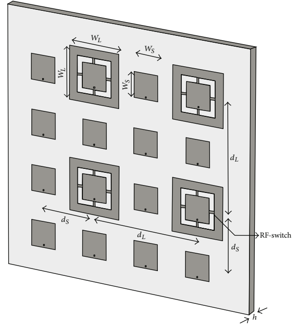
FIGURE 11: Reconfigurable ring-loaded patch antenna array [20].
