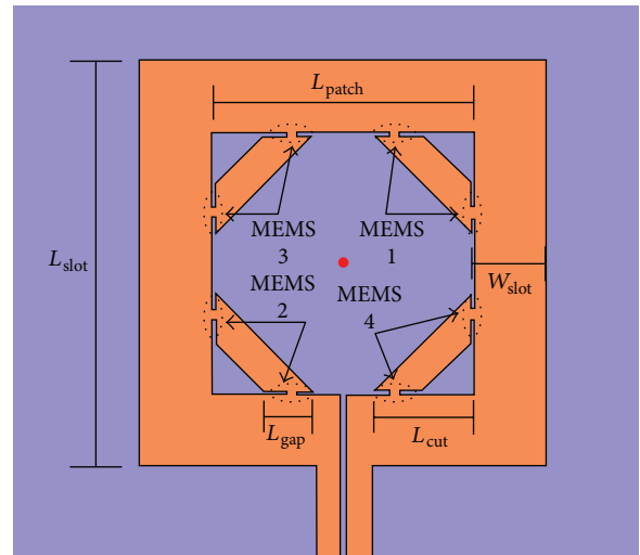
FIGURE 5: Frequency and polarization agile patch antenna [8].
