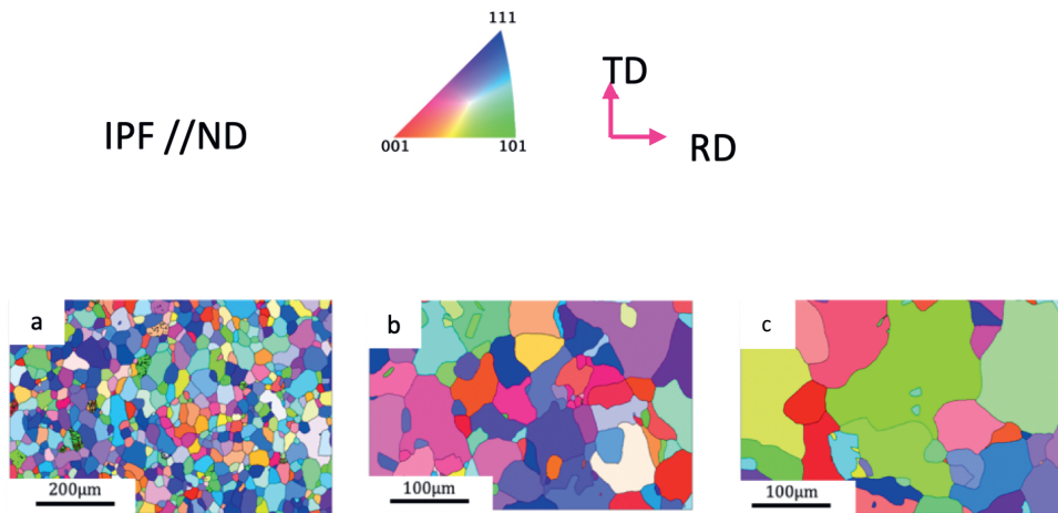
Figure 4.2 Microstructures obtained through EBSD measurements for all samples with different grain sizes. The Inverse Pole Figure (IPF) maps show the spatially resolved crystal directions parallel to the normal direction (ND) a) Sample S, b) Sample M and c) Sample L
