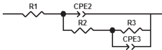
Figure 7.5 Equivalent circuit proposed for modelling the electrochemical response of dual-phase microstructures
