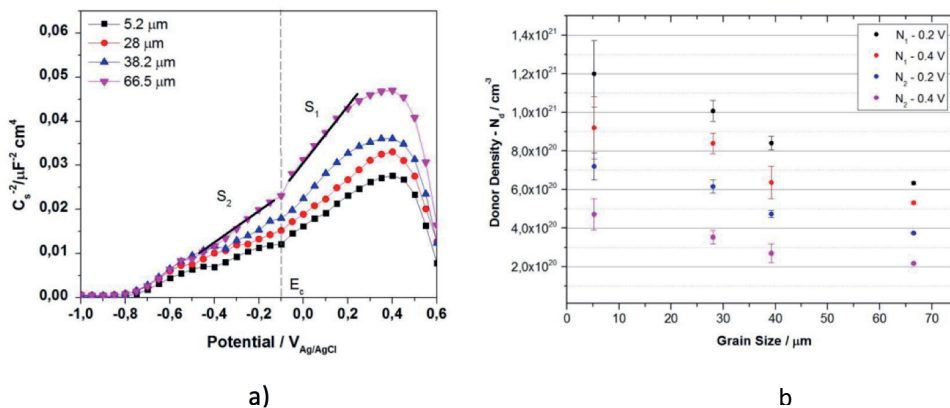
Figure 5.10 a) Mott-Schottky plot of samples after forming passive layer at 0.4 V (vs. \text{Ag}/\text{AgCl} ) for 6 hours. b) Donor density values of the passive layers formed at both 0.2 and 0.4 V (vs. \text{Ag}/\text{AgCl} ) for 6 hours
