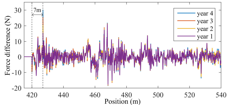
Figure 9. Contact force differences under singular local wear irregularity comparing with the reference force.
