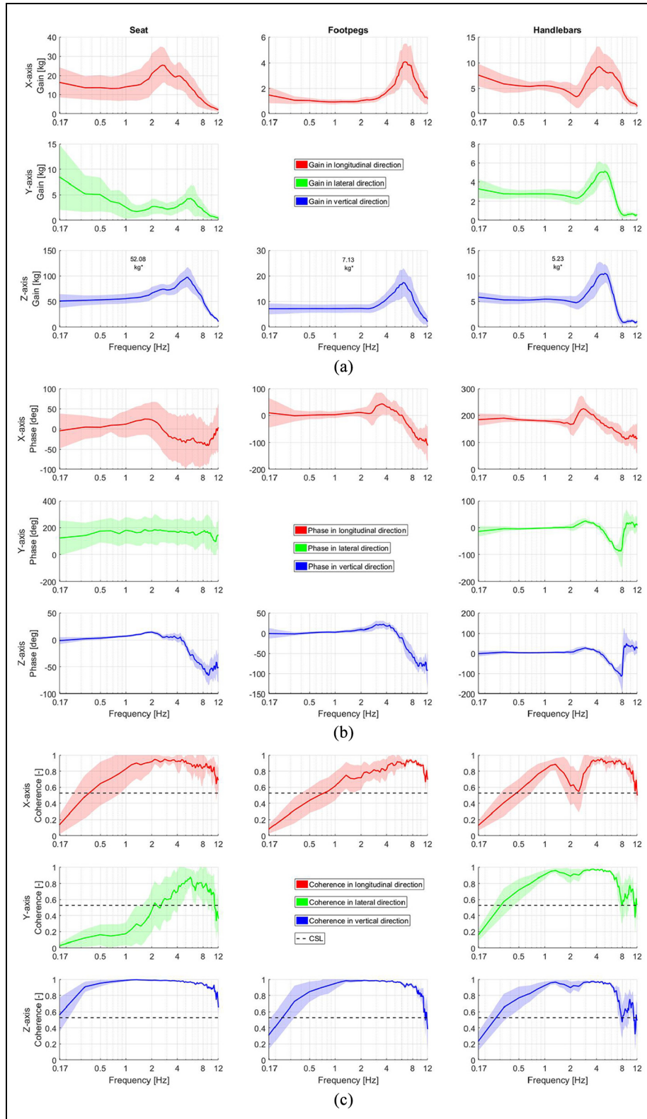
Figure 8. Apparent mass (APMS) for the heave (Z, vertical) motions as a function of the applied frequency (f) at the seat, footpegs, and handlebars: (a) magnitude, (b) phase, and (c) coherence, shade = standard deviation over participants. CSL = coherence significance level.
