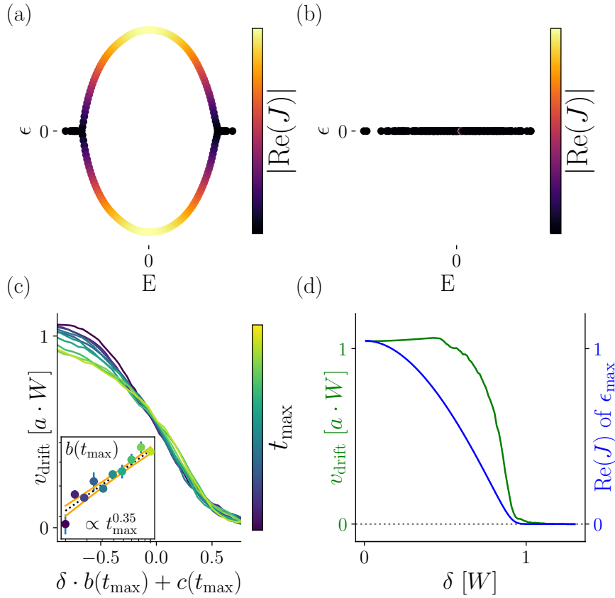
Figure 3: Finite-size scaling of the Hatano-Nelson Hamiltonian Eq. (1), with onsite disorder. Random disorder terms U_{i,j} with i \in \{0, 1, 2\} and j the site number (1) are sampled from distributions with standard deviation \delta_i . We set \delta_1 = \delta_2 = 0 and label \delta_0 as \delta . (a)-(b) The Hatano-Nelson spectrum for disorder strength (a) \delta = 0.3 and (b) \delta = 1.2 . (c) Rescaled wave packet drift v_{\text{drift}} at the transition point, collapsed using the relevant scaling parameter b(t_{\text{max}}) and the irrelevant scaling parameter c(t_{\text{max}}) . Inset: fit of the scaling parameter b(t_{\text{max}}) and the 95% confidence interval. (d) Comparison of v_{\text{drift}} (green) to \text{Re}(J) of \epsilon_{\text{max}} (blue) for system sizes L = 10^3 . Plot details in App. A.
