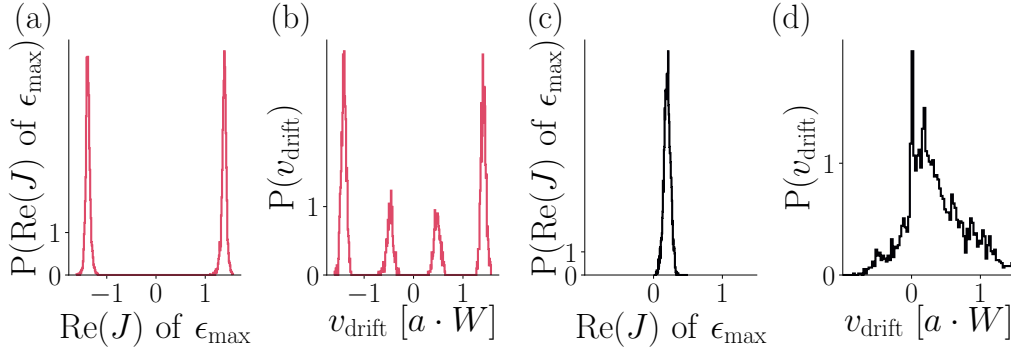
Figure 4: Multimodal and bimodal distributions of \text{Re}(J) and v_{\text{drift}} of the Hamiltonians H_{\infty} [Eq. (4)] and H_{\text{HN}} [Eq. (1)]. For the Hatano-Nelson Hamiltonian (1), random disorder terms U_{i,j} with i \in \{0, 1, 2\} and j the site number are sampled from distributions with standard deviation \delta_i . We set \delta_0 = \delta_1 = \delta_2 \equiv \delta . For the Hamiltonian H_{\infty} (4), random disorder terms U_{i,j} with i \in \{0, 1, 2, 3, 4\} and j the site number are sampled from distributions with standard deviation \delta_i . We set \delta_0 = \delta_1 = \delta_2 = \delta_3 = \delta_4 \equiv \delta . (a), (c) distributions of \text{Re}(J) of the maximally amplified state and v_{\text{drift}} of the H_{\infty} model at \phi = 0 and \delta = 0.1 . (b), (d) distributions of \text{Re}(J) of the maximally amplified state and v_{\text{drift}} of the H_{\text{HN}} model at \phi = 0 and \delta = 0.8 . Plot details in App. A.
