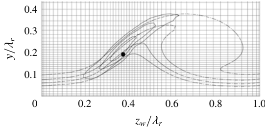
FIGURE 6. Zoom of mapped Chebyshev grid ( 55 \times 55 nodes). |\tilde{u}_w|/\max|\tilde{u}_w| of type I (solid contours at 25%, 50% and 75%). \bar{U}_w/\bar{U}_e levels 0.6, 0.7, 0.8 and 0.9 (dash-dotted). Position of (\bar{V}, \bar{W}_w) -field saddle point (solid circle).
