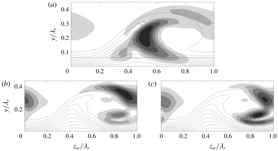
FIGURE 8. |\tilde{u}_w|/\max|\tilde{u}_w| for the type III mode ( a , in figure 7 a ) and the ‘harmonics’ of type II ( b, c , respectively II b , II c in figure 7 b ) modes, levels span [1/6, 5/6] with \Delta = 1/6 . Near-wall region (dash-dotted line). \bar{U}_w/\bar{U}_e levels 0.1, 0.2, \dots , 0.9 (dotted).
