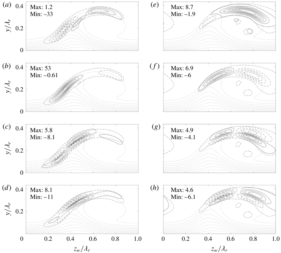
FIGURE 30. Imaginary part of the (a,e) R^y -, (b,f) R^{z_w} -, (c,g) A^{\bar{v}} - and (d,h) A^{\bar{w}} -integrands for type I (a–d) and II (e–h) on the weaker vortex (9 levels span (b) [-0.300, 47.2] , (c) [-0.873, 7.62] , (d) [-4.69, 5.59] , (e) [-6.74, 4.42] , (f) [-8.76, 6.21] , (g) [-3.20, 4.00] , (h) [-5.01, 3.56] , negative contours are dashed). Levels in (a) span [-27.8, -3.63] with \Delta = 4.84 , and [0.300, 0.900] , \Delta = 0.300 . All values are given in \bar{U}_e/\lambda_r^3 -units. Eigenfunction contour |\bar{u}_w|/\max|\bar{u}_w| = 1/6 (dash-dotted lines). \bar{U}_w/\bar{U}_e levels 0.1, 0.2, ..., 0.9 (dotted) for the weak vortex.
