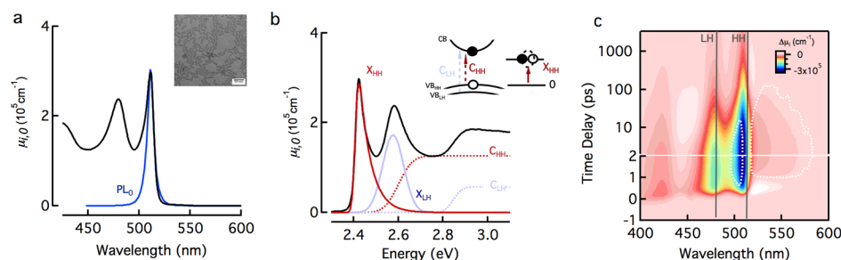
Figure 1. 4.5 ML colloidal CdSe quantum wells (a) PL (blue) and linear absorption spectrum (black) of the CdSe nanoplatelets dispersed in n -hexane, where the latter is normalized to represent the intrinsic absorption coefficient \mu_{i,0} . 48 Inset: TEM image showing an average lateral area of 34 \times 10 \text{ nm}^2 and no signs of stacking. (b) Absorption spectrum vs photon energy, decomposed into free carrier (C, dashed) and exciton (X, solid) contributions, both originating from the HH (red) and LH (blue) valence bands. Inset depicts the free carrier and exciton transitions. (c) Map of \Delta\mu_p , in \text{cm}^{-1} , for 400 nm photoexcitation creating \langle N \rangle = 84 as function of time (vertical axis) and probe wavelength (horizontal axis). The gray vertical lines indicate the position of the HH and LH exciton resonances. The white dashed contour indicates the regions where |\Delta\mu_p| > \mu_{i,0} , that is, where net optical gain occurs.
