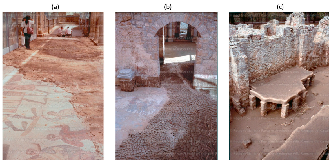
Fig. 6. Debris on the mosaics after 1991 debris flow (a): Corridoio della Grande Caccia (‘‘Ambulatory of the Big Hunting Scene’’); (b): Palestra (‘‘Fitness room’’); (c): Calidarium (‘‘Warm room’’). The absence of the floor and the bottom of the hollow space at a lower level makes the room easy to be flooded (source: www.villaromanelcasale.it ).
