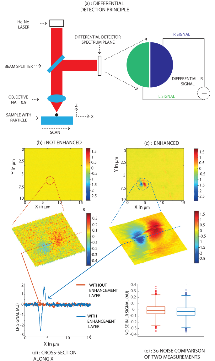
FIG. 3. The differential detection principle is shown in panel (a). In panels (b) and (c) the far-field maps of the sample without and with the enhancement layer are shown. The figures under panels (b) and (c) show the three-dimensional view of the signal maps near the particle. Please note the change in scale for the not-enhanced case, which is necessary to show the signal from the particle. (d) Signals can be quantitatively compared by plotting the cross sections. The noise of the two measurements are compared in panel (e), which have mean +3\sigma \approx -0.09 + 0.42 (without enhancement layer) and -0.2 + 0.42 (with enhancement layer). Particle localization is not possible without the enhancement layer.
