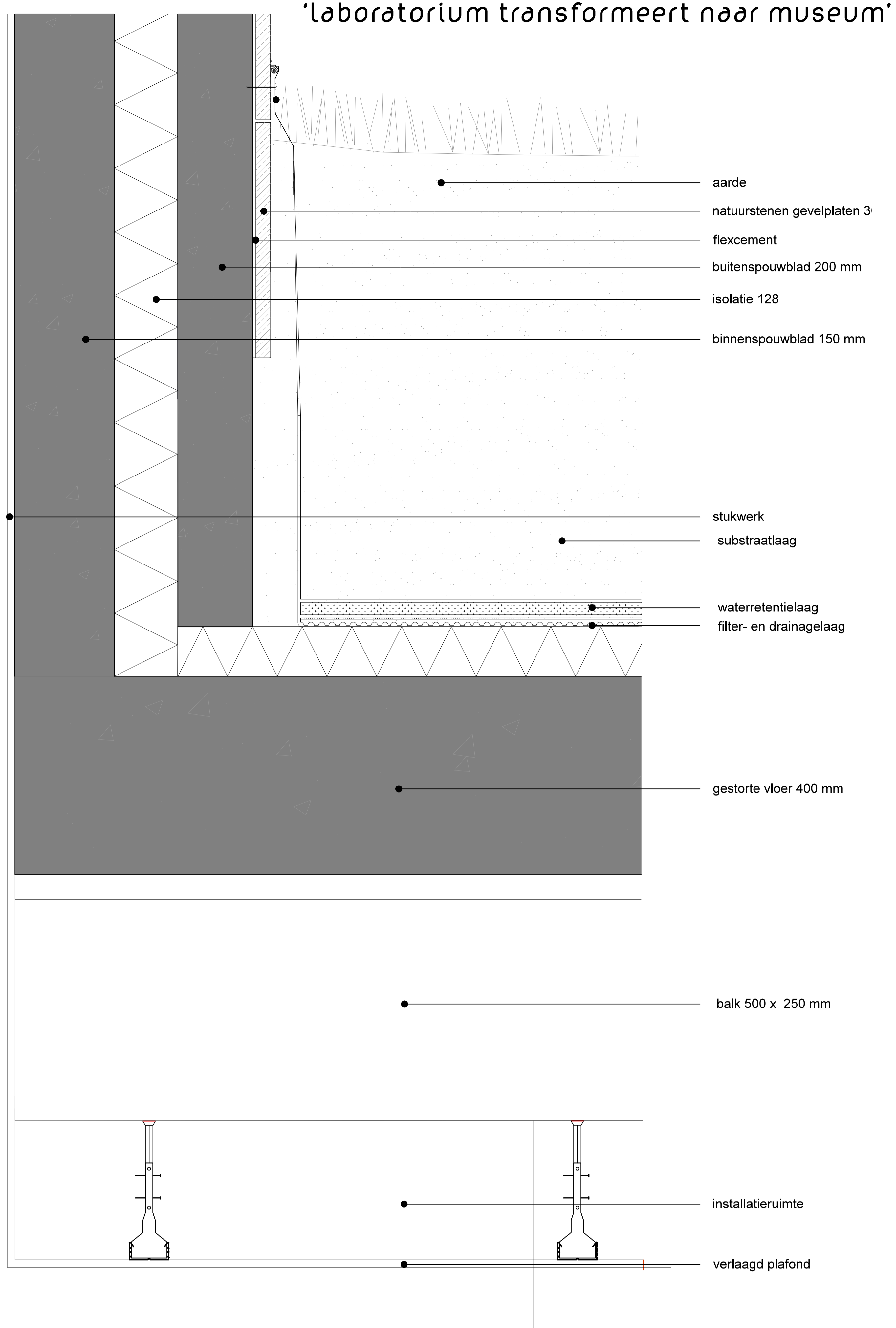
detail 4. _ 1:5
