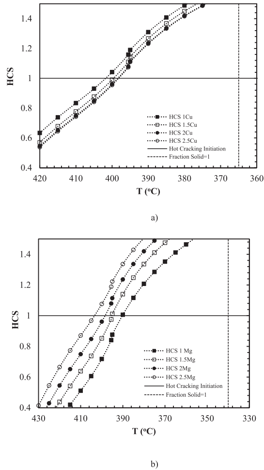
Fig. 6. The HCS curve based on SKK criterion (a) Al9Zn2Mg(1, 1.5, 2, 2.5%wt.)Cu, and (b) Al9Zn(1, 1.5, 2, 2.5%wt.)Mg2Cu.
