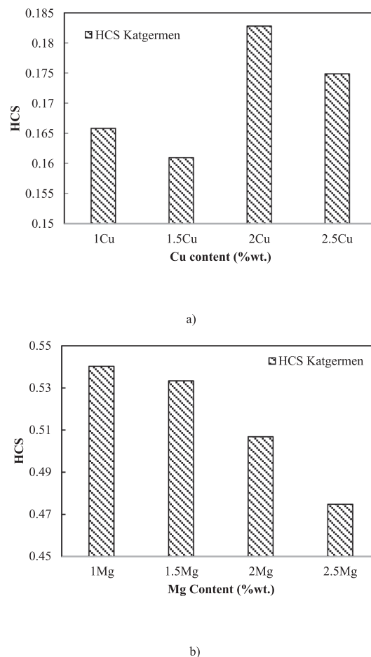
Fig. 5. The HCS curve based on Katgerman criterion, (a) Al9Zn2Mg(1, 1.5, 2, 2.5 %wt.)Cu, and (b) Al9Zn(1, 1.5, 2, 2.5 %wt.)Mg2Cu.
