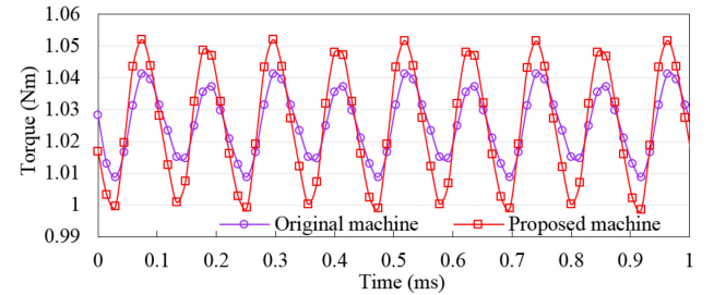
Fig. 8. Torque waveforms of the original and new machines with 25 A phase current.
