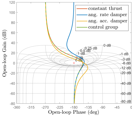
Fig. 5. Nichols plot for three strategies. Constant thrust and the control group overlap. The angular rate damper strategy should provide the best stability.
