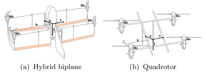
Fig. 2. Drawings of the hybrid biplane and quadrotor with body axis definitions. The control surfaces are accentuated in light orange.
