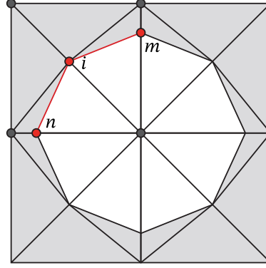
Fig. 20. Line elements ni and im (marked with red segments) sharing node i are used to compute the outward normal \mathbf{n}_i of node i .
