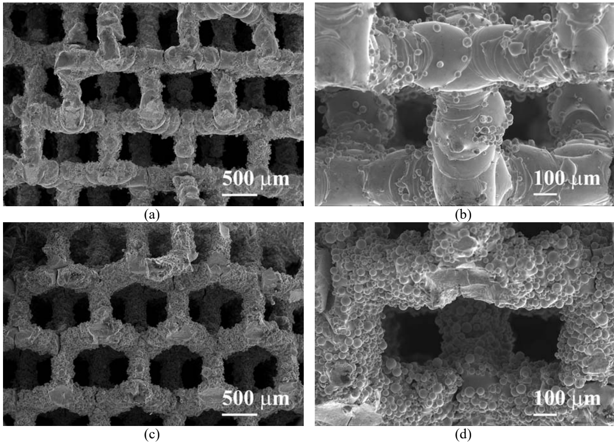
Figure 2- Strut surface morphology of selective laser melted (a) Co-Cr (magnification: X30), (b) Co-Cr (magnification: X100), (c) Ti-6Al-4V (magnification: X30), and (d) Ti-6Al-4V (magnification: X100) porous structures based on diamond unit cell
