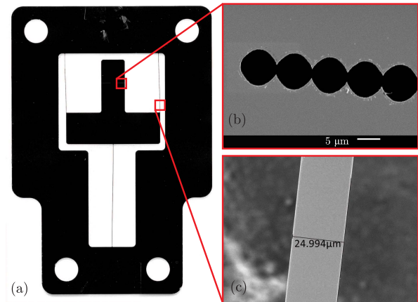
Fig. 9. Micrographs of a balanced stage. (a) A picture of a balanced stage. It can be observed it is buckled in the mode from Fig. 5b. (b) A SEM image of the markers used to align the microforce sensing probe with the center of compliance, see Fig. 4b. In figure (c) a typical SEM image used for measuring the beam width is shown.
