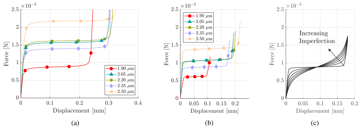
Fig. 6. Simulation results for statically balanced stages (a) with (b) and without oxide for multiple oxide thicknesses. (c) Shows the influence of beam imperfections on the force deflection response for the stage where 2.35 \mu\text{m} of \text{SiO}_2 has been removed.
