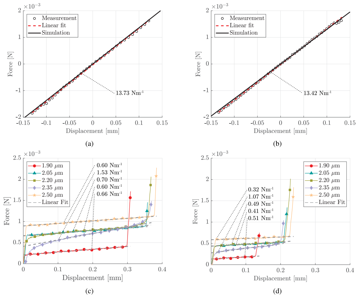
Fig. 10. Force deflection measurements averaged over 10 repetitions to reduce constant measurement noise. (a) A typical measurement with linear fit along with a simulation of an unbalanced oxidized stage. (b) A typical measurement with linear fit along with a simulation of a non-oxidized unbalanced stage. (c) Measurements of the balanced devices with \text{SiO}_2 with a linear fit to the low stiffness domain. (d) Measurements of the balanced devices with \text{SiO}_2 removed with a linear fit to the low stiffness domain.
