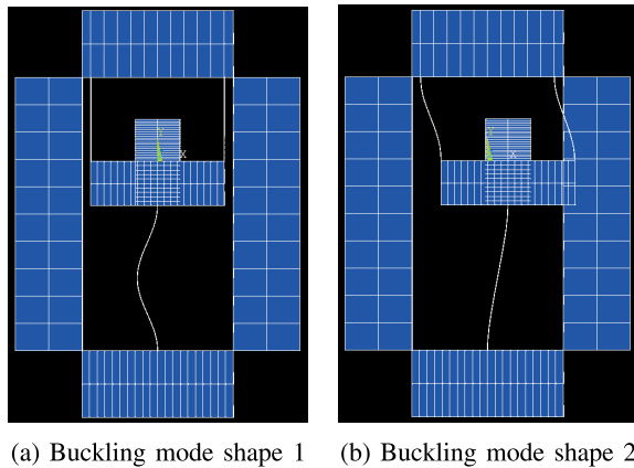
Fig. 5. The first two buckling modes resulting from uniformly cooling down the sample. Modeling is done as described in Section V.
