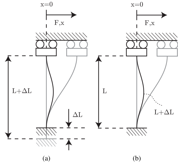
Fig. 2. Commonly used compliant equivalent of the balancer from Fig. 1. (a) Shows preloading by moving the end point of the plate spring a distance \Delta L . (b) Shows preloading by stretching the plate spring a distance \Delta L . Both systems are equivalent.
