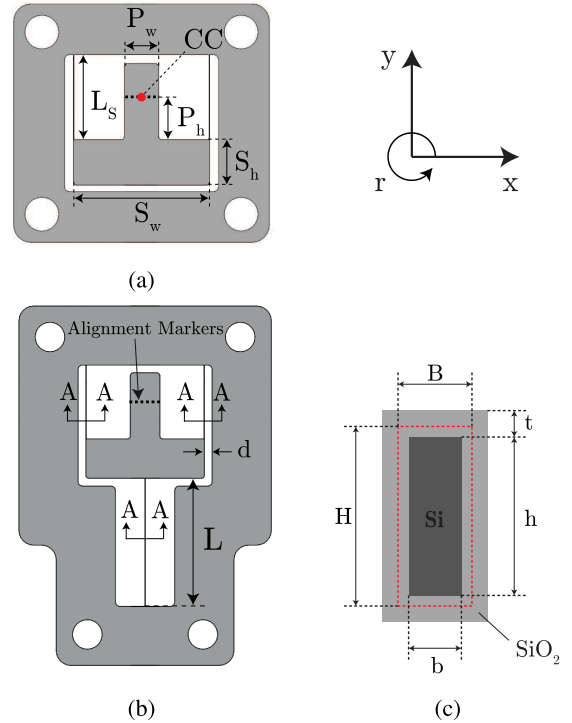
Fig. 4. Stage designs. (a) Shows the unbalanced stage and (b) the balanced stage. (c) Shows the cross section A-A of the plate springs, which is the same everywhere. The dashed rectangle indicates the silicon beam before some of its material is consumed by oxidation.
