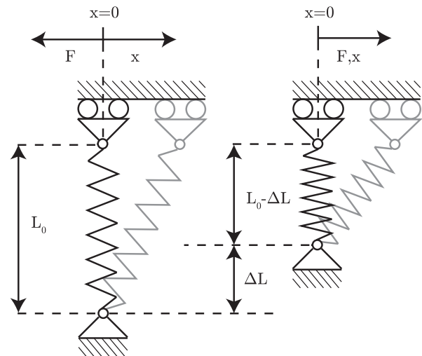
Fig. 1. Balancer with negative stiffness used for static balancing, comprised of a compression spring with free length L_0 on a cart. In the unloaded configuration (left), displacement of the cart results in a returning force to the stable equilibrium at x = 0 . If preloaded a distance \Delta L , displacement of the cart results in a force away from the unstable equilibrium at x = 0 , i.e. negative stiffness.
