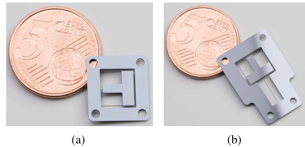
Fig. 8. Manufactured stages. (a) Shows the unbalanced stage and (b) shows the balanced stage.
