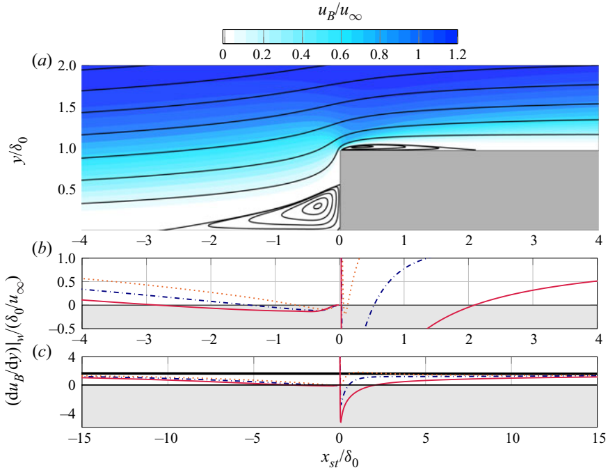
Figure 9. (a) Base-flow chordwise velocity (colour map) with lines of constant streamfunction (solid black). (b,c) Wall shear (du_B/dy)|_w : smooth case (thick solid black), step case I (dotted orange), step case II (dash-dotted blue), and step case III (thin solid red).
