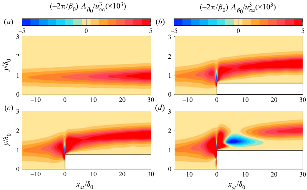
Figure 20. Integrand of the Reynolds–Orr production term P_{\beta_0} in (a) the smooth case, (b) step case I, (c) step case II, and (d) step case III.
