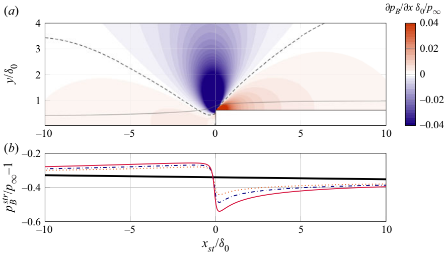
Figure 5. (a) Base-flow chordwise pressure gradient (colour map) \partial p_B / \partial x = 0 (black dashed line), projected base-flow streamline seeded at x/\delta_0 = 0, y/\delta_0 \approx 0.2 (grey solid line) in step case II. (b) Static pressure along the streamline in the smooth case (thick solid black), step case I (dotted orange), step case II (dash-dotted blue), and step case III (thin solid red).
