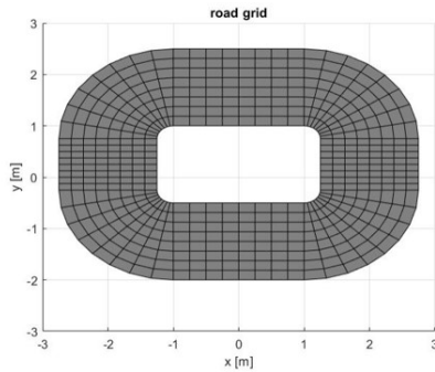
Fig. 1. Road grid made out of a combination of grid points that are connected.
