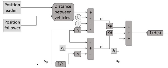
Fig. 4. Implementation of a CACC.
