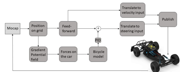
Fig. 3. Control scheme of the leader car (Erle-Rover with Erle-Brain [17]).
