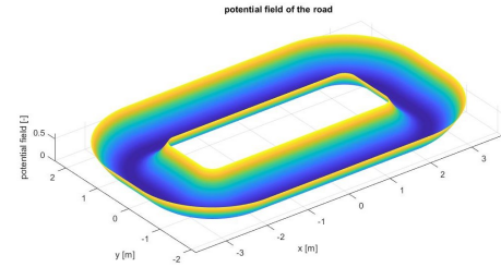
Fig. 2. Static potential field.
