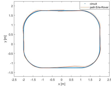
Fig. 5. Standard circuit, single Rover experiment ( A_r = 20 , b_r = 0.30 ).
