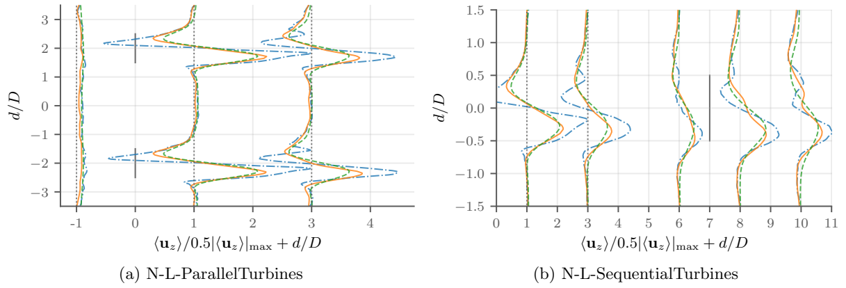
Figure 7: Normalized \langle \mathbf{u}_z \rangle profile for N-L-ParallelTurbines and N-L-SequentialTurbines at z_{\text{hub}} using LES (— · —), RANS with b_{ij}^{\text{LES}} injection (—), and baseline RANS (— · —).
