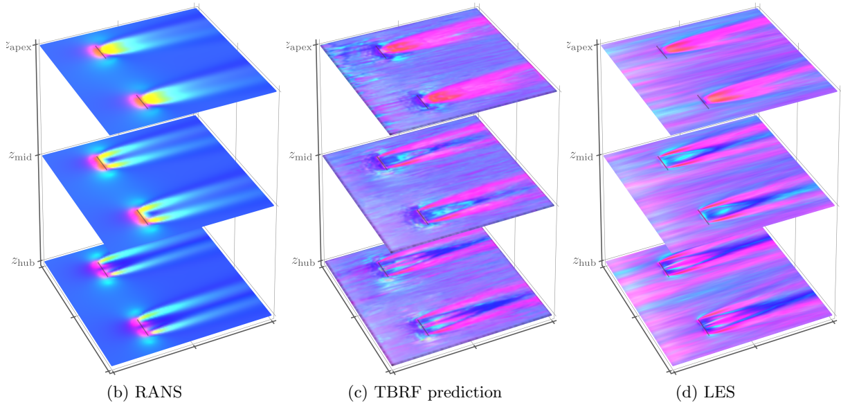
Figure 8: Barycentric map at z_{\text{hub}} , z_{\text{mid}} , and z_{\text{apex}} for N-H-ParallelTurbines using RANS, TBRF prediction after training on the N-H-OneTurbine LES ground truth, and LES
