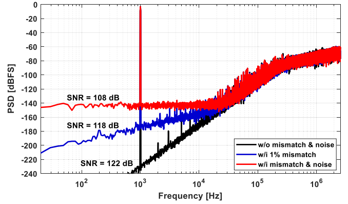
Fig. 3. Output spectra of the CT zoom ADC with different error sources.
