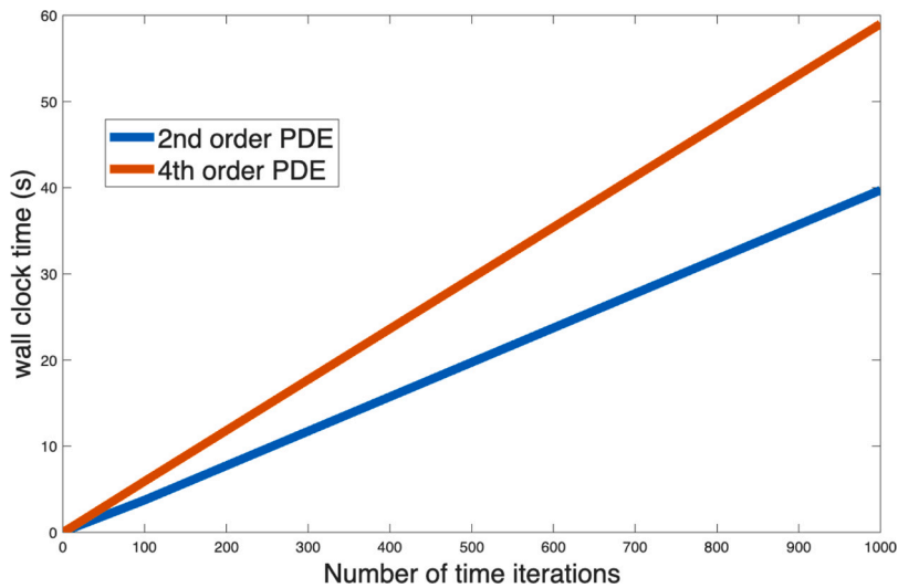
Fig. 5. Computation times (wall clock times) using tic-toc in Matlab for a second and fourth order PDE.
