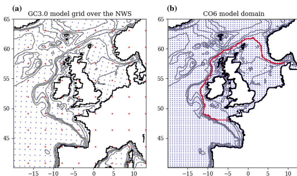
Fig. 2 GC3.0 and CO6 model grids, showing model coastline (black), depth contours (at 50, 100, 200, 500, 1000 and 2000 m, grey), and every 5th ocean grid box (blue dots). a the GC3.0 model grid, also showing every 5th atmosphere grid box (red dots). b CO6 model domain, also showing the extent of the NWS (red)—it is (approximately) delineated by the 200 m isobath, but excludes the Armorican shelf, the Skagerrak/Kattegat and the Norwegian Trench
