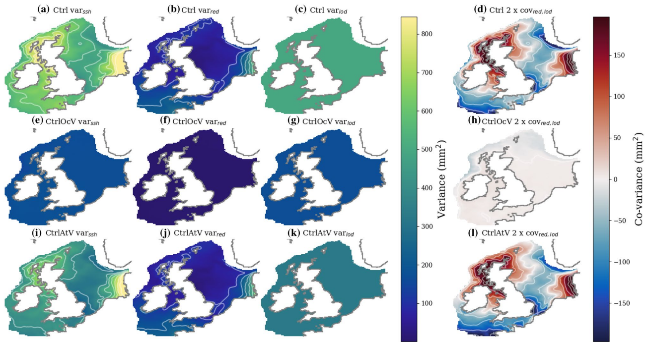
Fig. 9 The left hand column is the total variance ( var_{ssh} : a , e , i ), the second and third column is the variance associated with the redistribution ( var_{red} : b , f , j ) and loading term ( var_{lod} : c , g , k ) respectively, with (two times) their covariance in the right hand column ( 2 \times cov_{red,lod} : d , h , l ). The total variance ( var_{ssh} ) is the exact sum of the variance associated with the redistribution and loading and two times their covariance ( var_{red} , var_{lod} and 2 \times cov_{red,lod} ). The vari-
