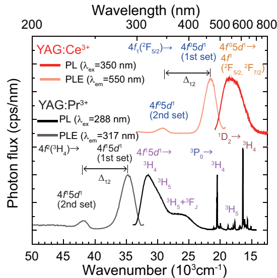
FIG. 2. PL and PLE in \text{Y}_3\text{Al}_5\text{O}_{12} doped with 0.2% \text{Pr}^{3+} and 0.1% \text{Ce}^{3+} .
