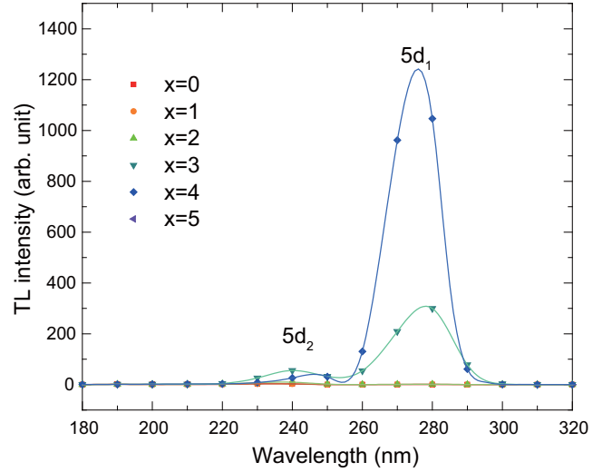
FIG. 7. Integrated TL intensity between 300 K and 600 K as a function of charging excitation wavelength from 180 nm to 320 nm with 300 s charging time in \text{Y}_3\text{Al}_{5-x}\text{Ga}_x\text{O}_{12} : \text{Pr}^{3+} .
