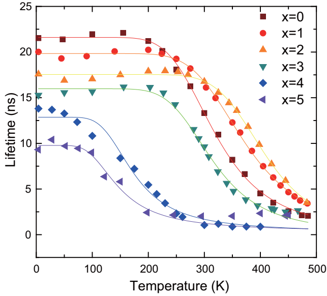
FIG. 6. Temperature dependence of lifetime in \text{Y}_3\text{Al}_{5-x}\text{Ga}_x\text{O}_{12} : \text{Pr}^{3+} .
