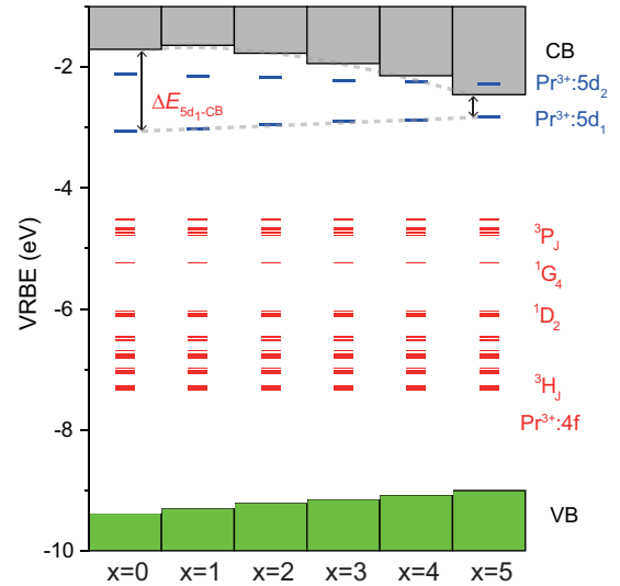
FIG. 9. Stacked VRBE diagram of \text{Y}_3\text{Al}_{5-x}\text{Ga}_x\text{O}_{12}:\text{Pr}^{3+} .
