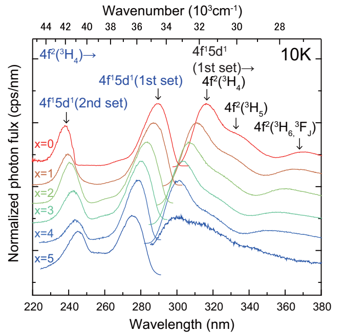
FIG. 3. PL (for excitation to the 5d_1 state) and PLE (for 5d_1-4f luminescence) of \text{Y}_3\text{Al}_{5-x}\text{Ga}_x\text{O}_{12}:\text{Pr}^{3+} ( x = 0, 1, 2, 3, 4 ) at 10 K. For the x = 5 samples, PLE was measured by monitoring ^3P_J luminescence.
