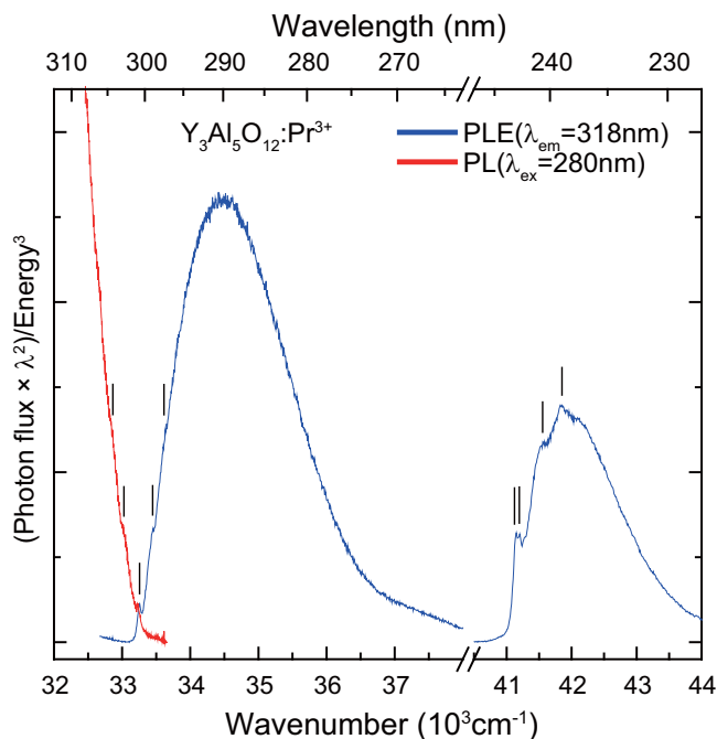
FIG. 4. High-resolution PL spectrum (excited by 280 nm) and PLE spectrum (of 318 nm luminescence) in \text{YAG:0.2\%Pr}^{3+} at 8 K. Vertical black lines are phonon lines.
