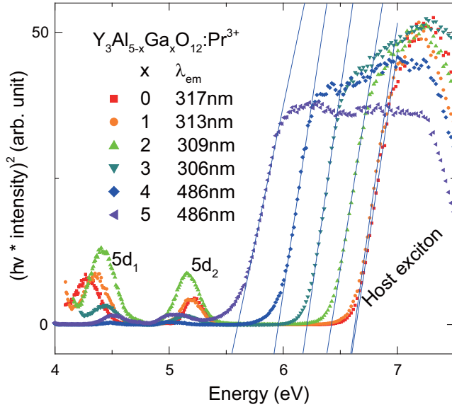
FIG. 8. Tauc plot of PLE spectra in the VUV region in \text{Y}_3\text{Al}_{5-x}\text{Ga}_x\text{O}_{12}:\text{Pr}^{3+} .
