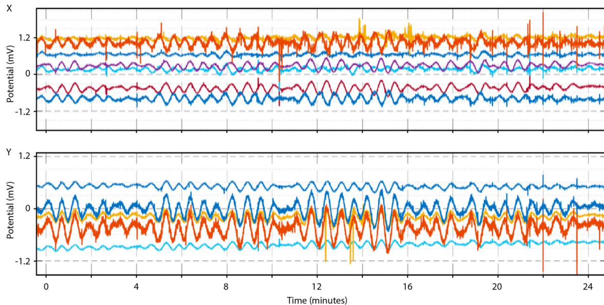
Figure 1. Time series of the electric potential for a geophysical study. Shown are simultaneous recordings at many separate locations (colors). Measurements were made with the porous-pot electrodes discussed here (type 1). The fields were recorded in two orthogonal horizontal directions (X, north–south; Y, east–west), with 60m dipole lengths. For the magnetotelluric technique, electric field data are combined with simultaneous magnetic field recordings. Data come from measurement locations in the Khovsgol region of northern Mongolia, approximately 50°N and 100°E (Rigaud, Comeau, Becken, et al., 2023, Rigaud, Comeau, Kuvshinov, et al., 2023): n6120, n6100, n6160, n8060, n8070, n8080, n8100, n8105, and s030. Geomagnetic pulsations are observed (Pc3, about 40s period). The sampling rate shown here is 8Hz. Time is measured in minutes from 9:40:0 16 August 2022.
