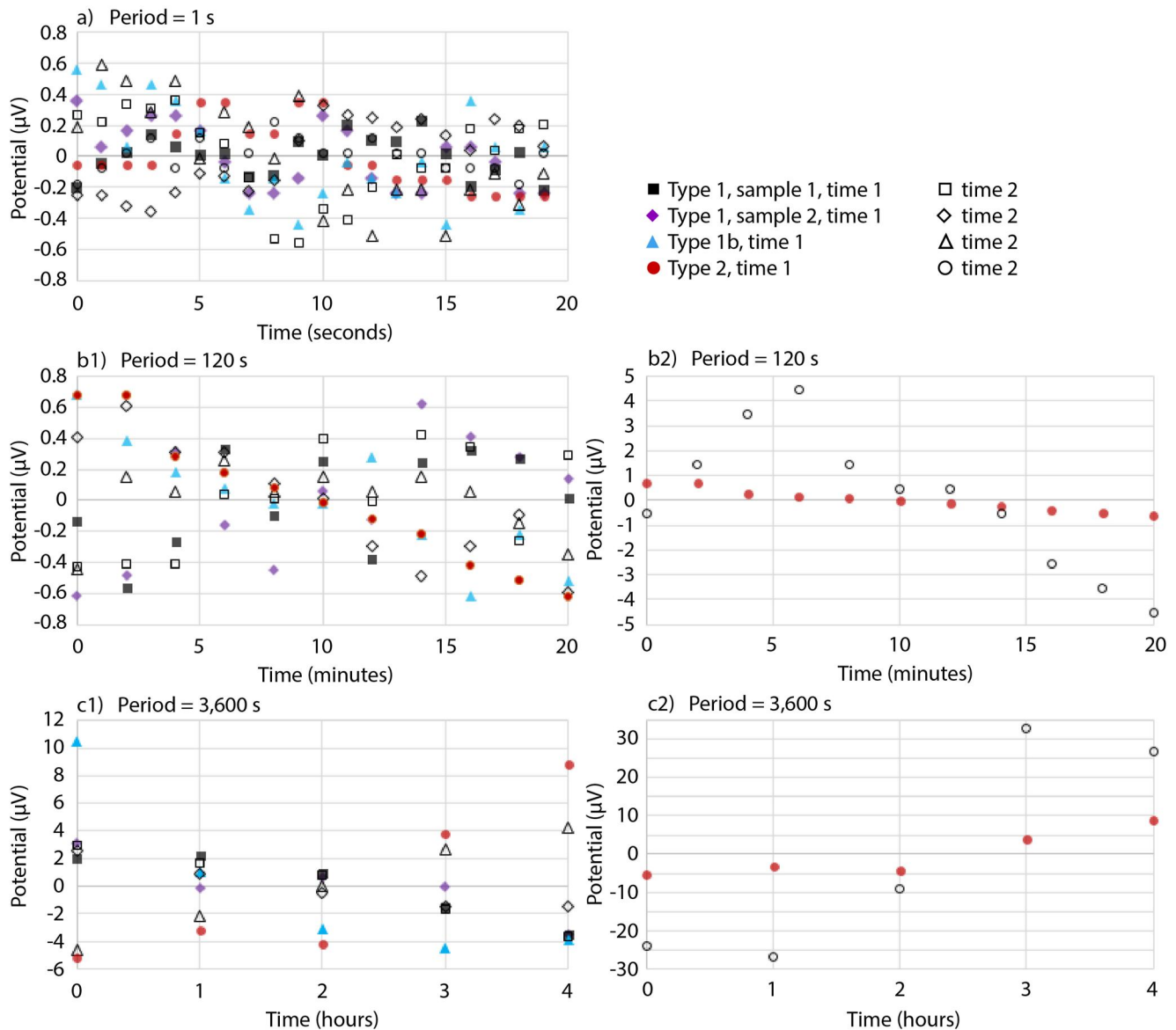
Figure 14. The difference of the electric potential measurements and the mean over selected periods for different types of electrodes. (a) Measurements taken 1 s apart; (b) Measurements taken 120 s apart (second panel for type 2 electrodes due to change of axis scale); (c) Measurements taken 3,600 s apart (second panel due to change of axis scale). Symbol denotes electrode type; the symbol fill is for the measurement run carried out at a different time, color fill for time 1 and empty fill for time 2. Electrode pair with (i) electrolyte and clay formula and ceramic porous plugs (type 1; #012–21) shown with diamonds (purple), ii) electrolyte and clay formula and ceramic plugs (type 1; #9–48) shown with squares (black), iii) electrolyte and clay formula and wood plug (type 1b; #W1–W2) shown with triangles (blue), iv) electrolyte-only (no clay) and ceramic plugs (type 2; #L1–L2) shown with circles (red). Time 1 is measured from midnight 14 December 2022 and time 2 is measured from midnight 17 December 2022. At short periods (e.g., 1 s) the variations are small for all electrode types; at longer periods (e.g., 3,600 s) they become larger. Note the unit is \mu\text{V} , which is 0.001 mV.
