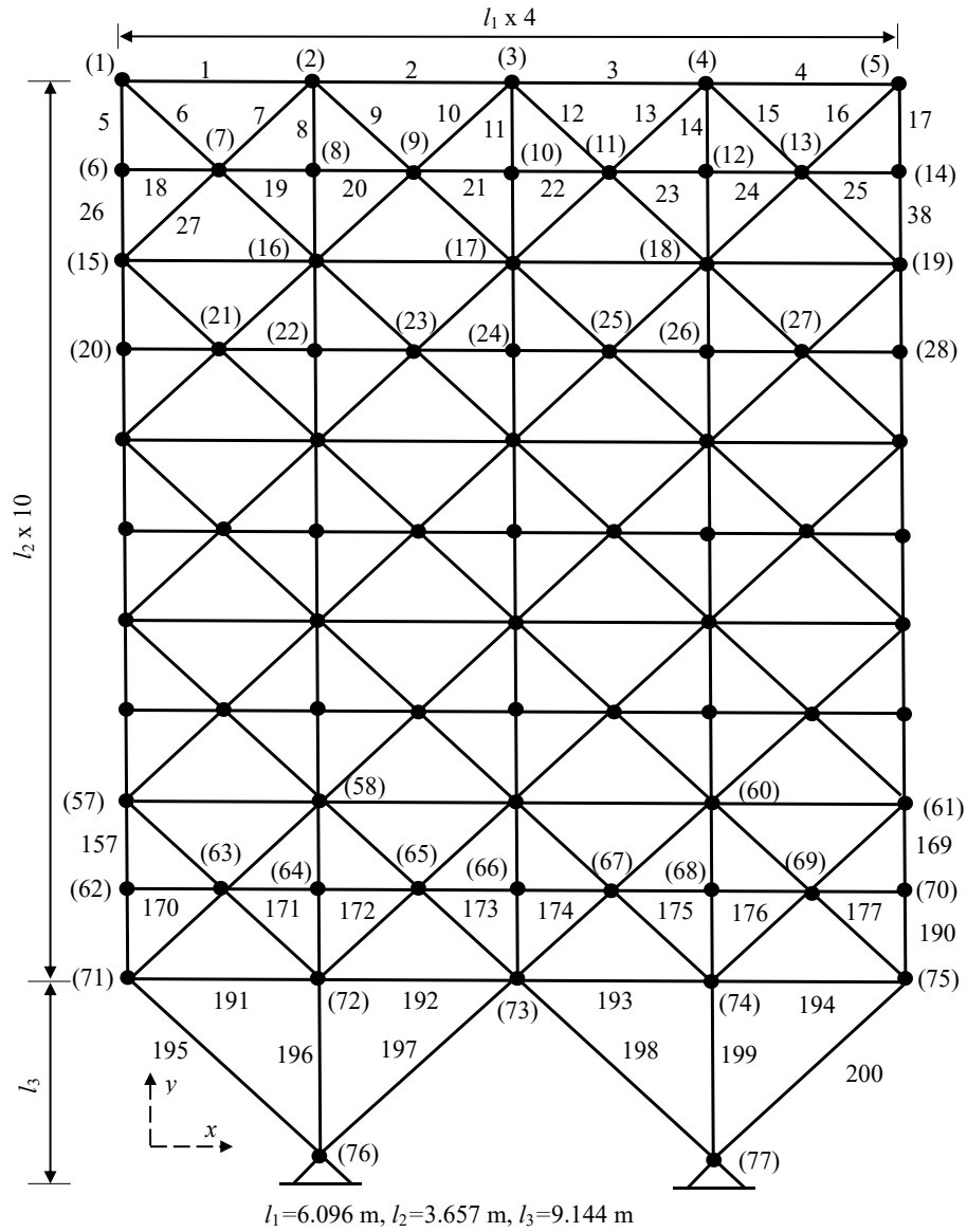
Figure 11. A 200-bar planar truss structure.
