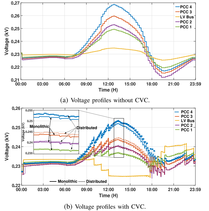
Fig. 5. Results of CVC using GDS setup [29].
