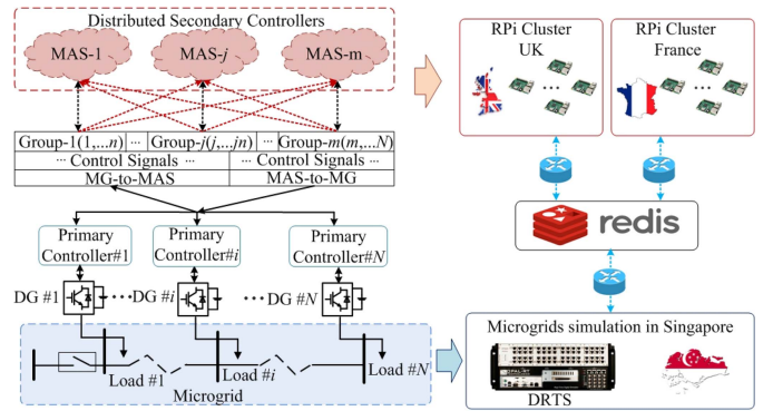
Fig. 6. RT-GD-CHIL setup for frequency and voltage control of microgrids [25].
