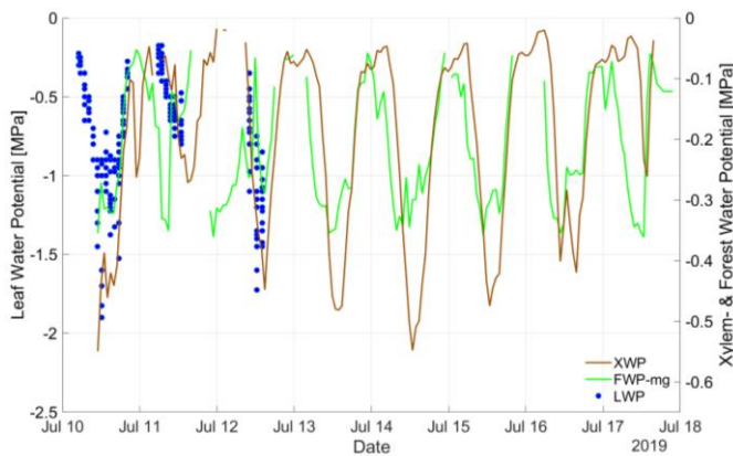
Fig. 6. Comparison of in situ measurements (xylem water potential: brown curve; leaf water potential: blue dots) and radiometer-based estimates (green curve) of FWP , assuming a static FWP_{min} .
