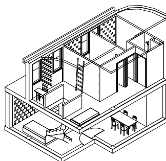
penthouse I 72 m 2
