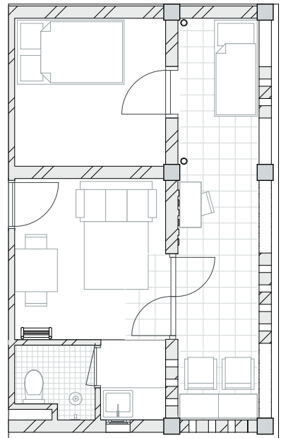
main floor
