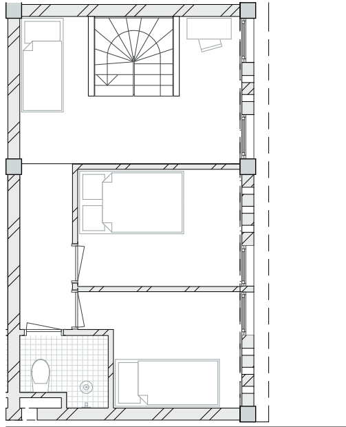
upper floor
