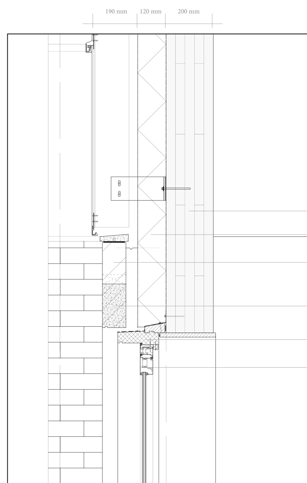
Facade detail 1.10
