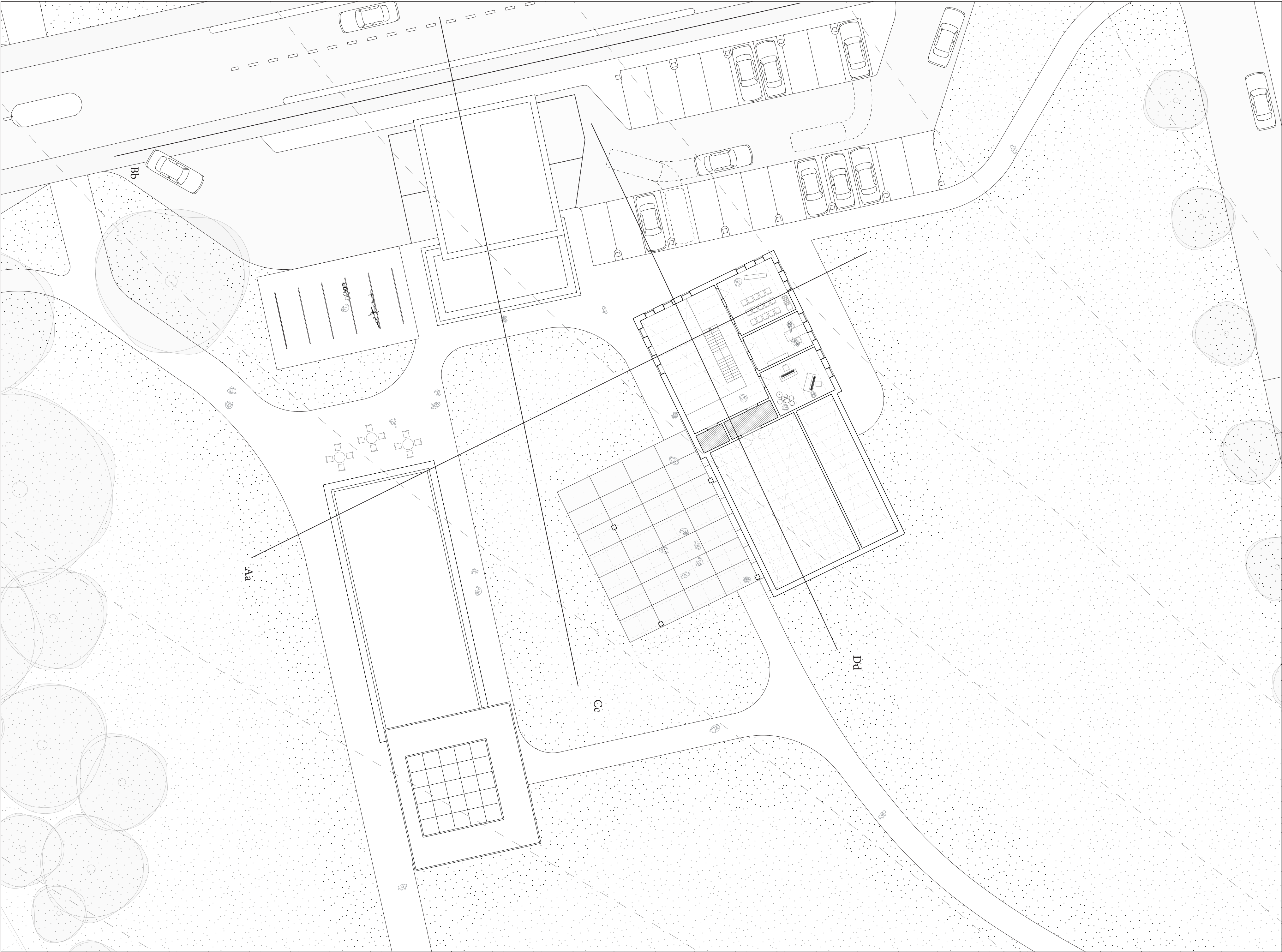
Plan first floor in context 1.200
