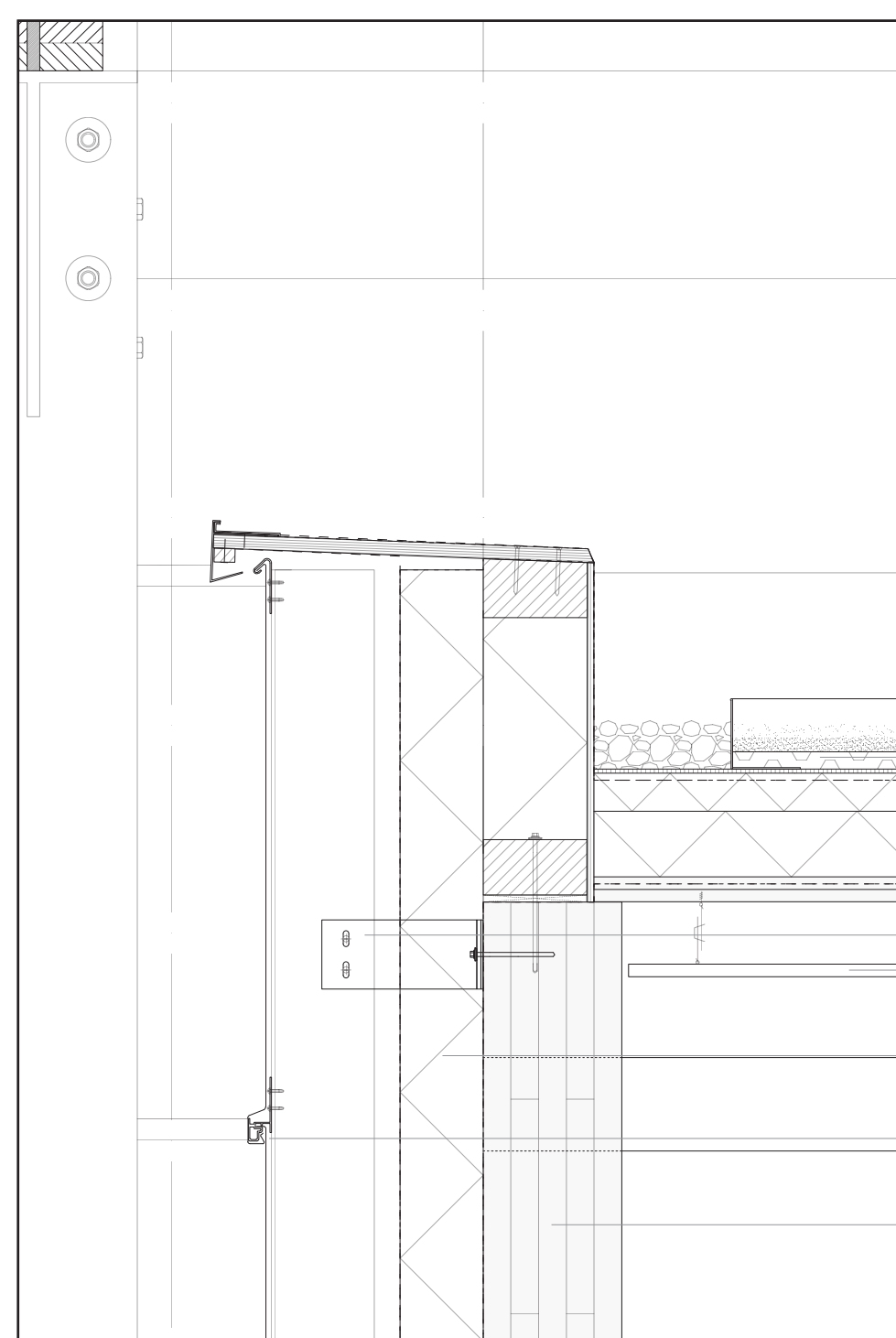
Roof detail 1.10
