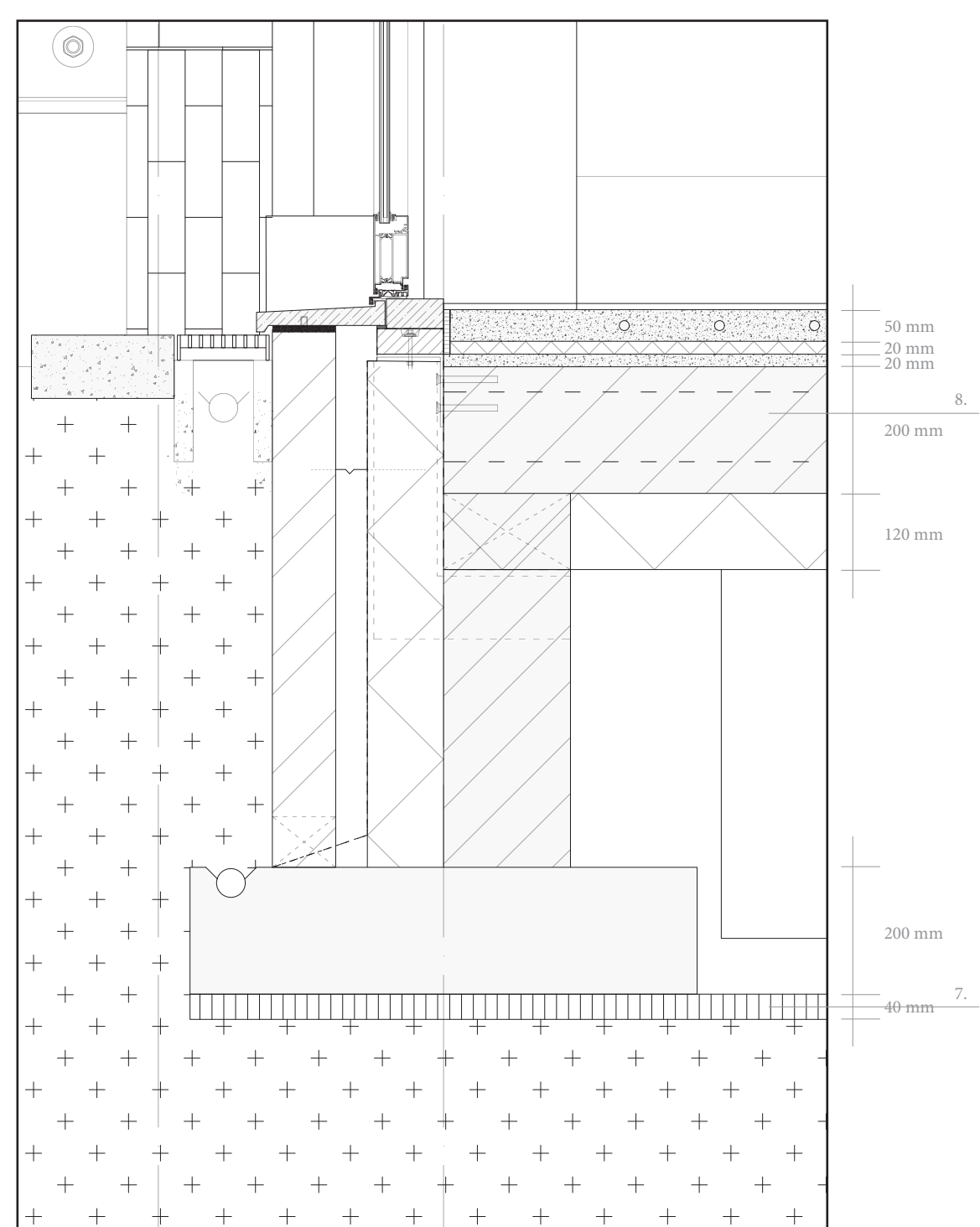
Foundation detail 1.10
