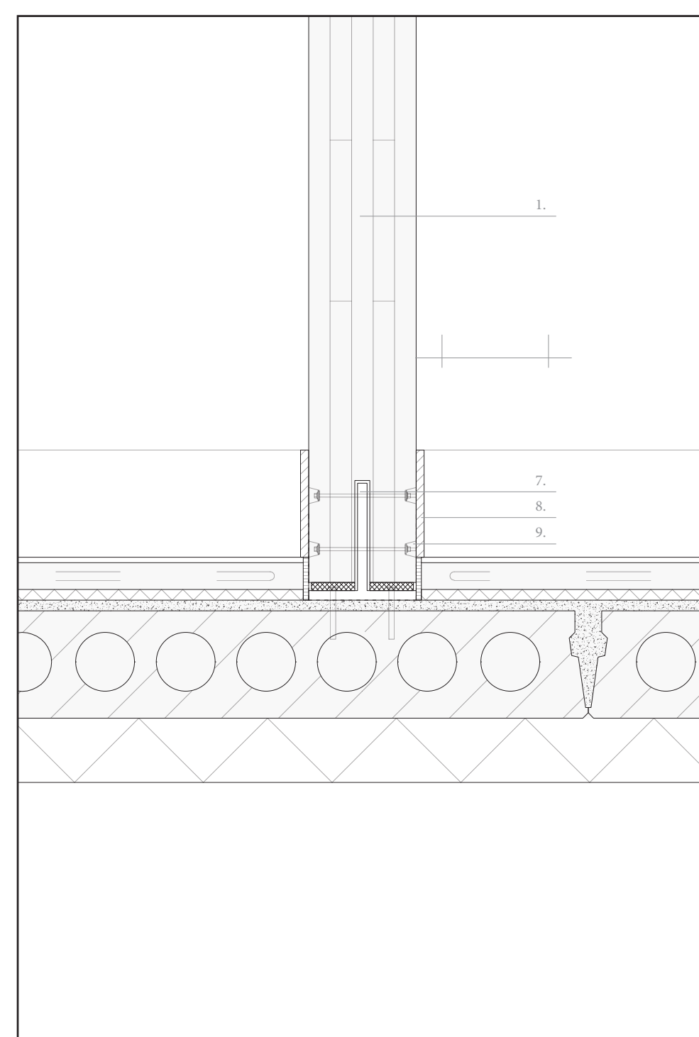
Interior CLT wall and floor detail 1.10
