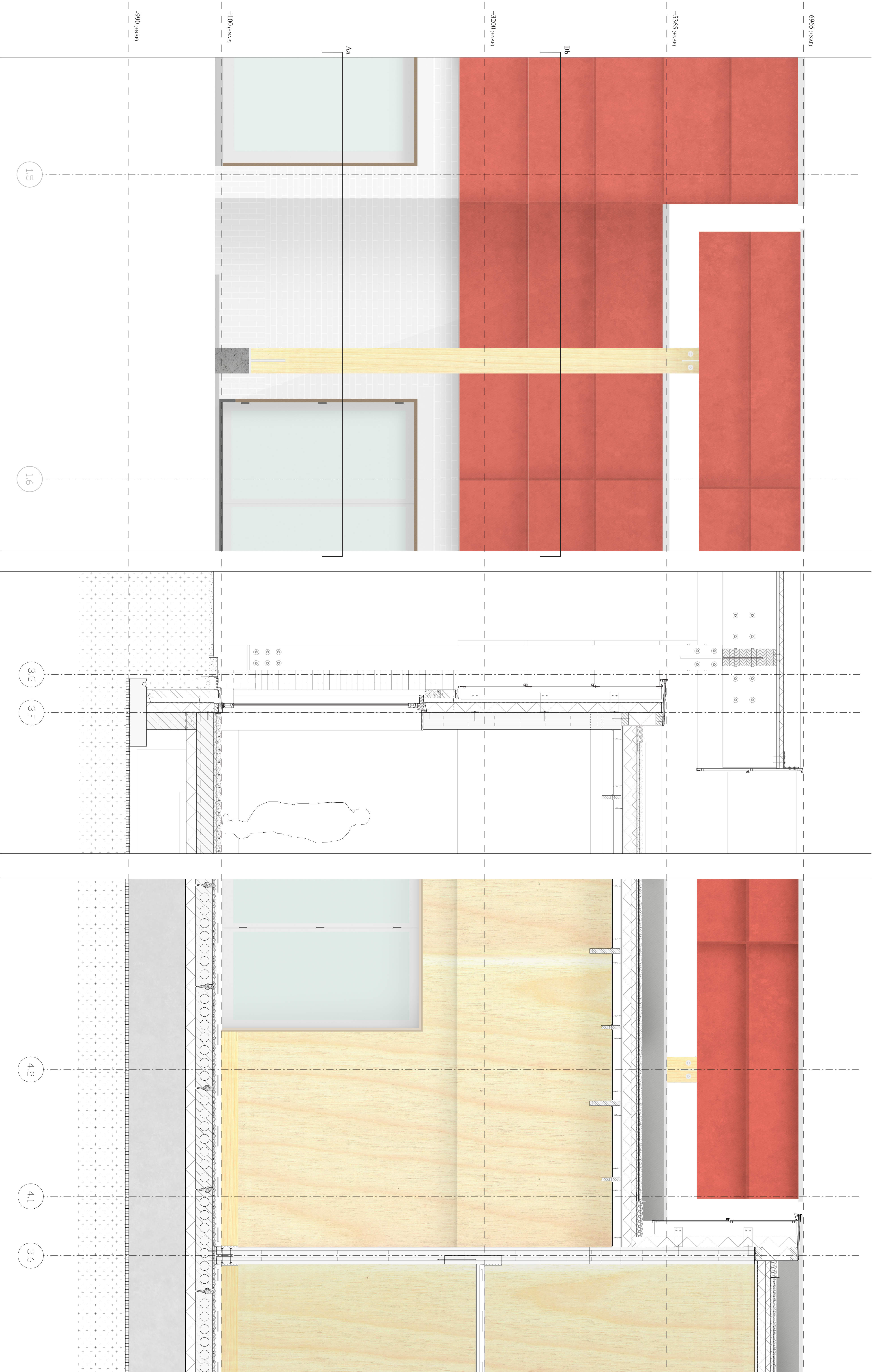
elevations and section of representative facade 1.20
