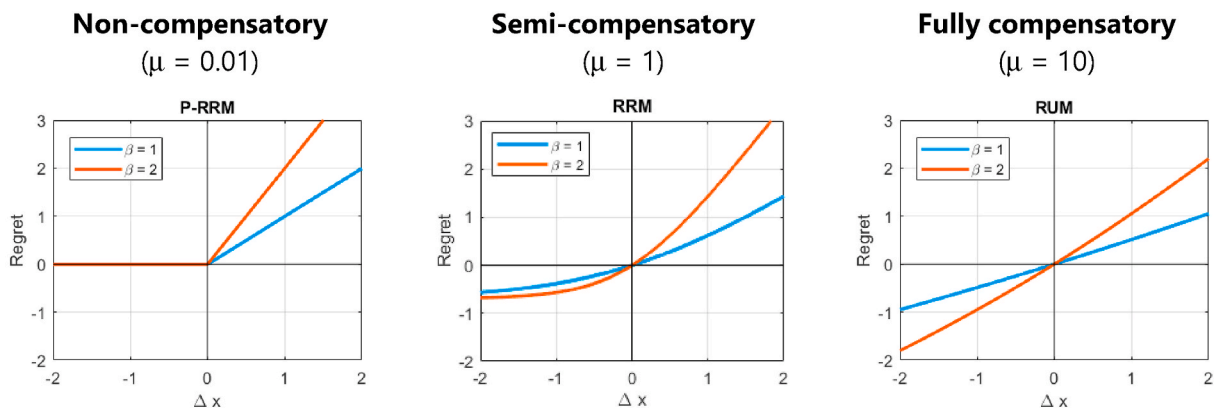
Δx means the difference in performance of two alternatives on an attribute. A positive value means the observed alternative (i) is performing worse than the comparing alternative (j), and vice versa (the model formulation is x_{jk} - x_{ik} ).
