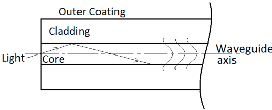
Figure 2.2: Components of a typical optical fibre.
