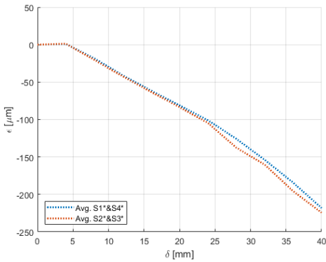
Figure 6.10: Strain trend in the bottom section of the wing undergoing bend-down with respect to deflection due to morphing.
