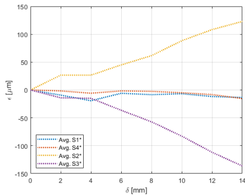
Figure 6.12: Strain trend in the bottom section of the wing undergoing twist with respect to deflection due to morphing.
