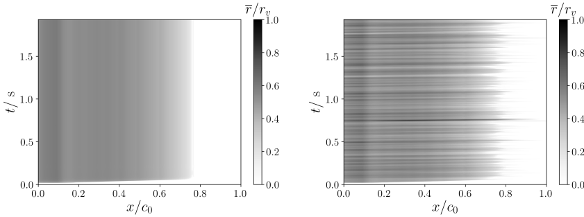
Figure 7.13: Space-time diagram of cavity radius normalised with viscous core radius. Left IDDES without ITG ( \mathcal{J}_{tip} = 0.0\% ), right with ITG ( \mathcal{J}_{tip} \approx 1.3\% ).
