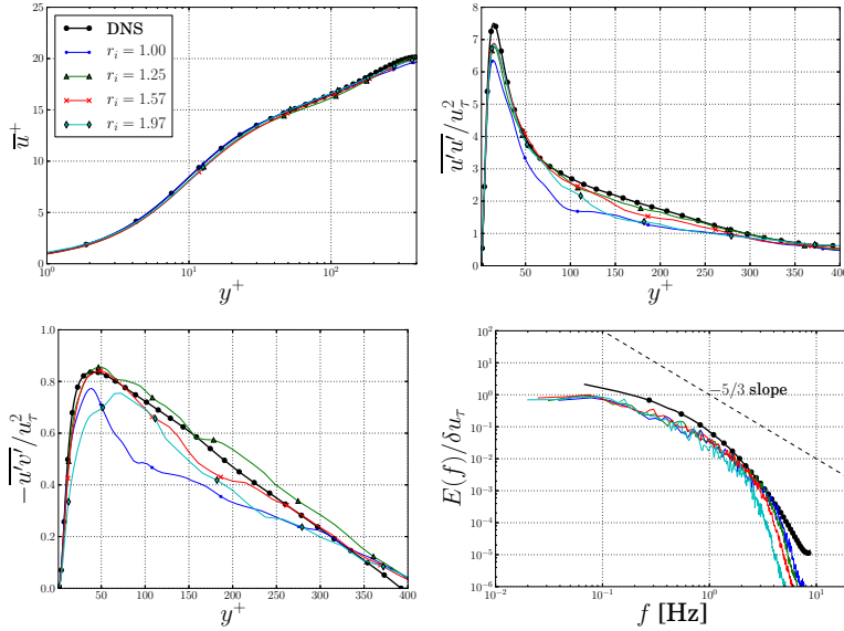
Figure 5.4: Mean velocity ( \overline{u}^+ ) profiles, Reynolds stress ( Re_{uu} and Re_{uv} ) profiles and turbulence kinetic energy spectra ( E_{u,y^+ \approx 20}(f) ) using different grids and PANS ( f_k = 0.10 ).
