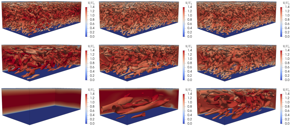
Figure 4.5: Instantaneous turbulent flow fields ( Q = 0.7 ), coloured by \bar{u}^* = \bar{u}/U_b . From left to right f_k = 0.15 , 0.10 and 0.05, for f_\epsilon = 1.0 (first row), f_\epsilon = 2 \cdot f_k (second row) and f_\epsilon = f_k (third row). Re_\tau = 395 .
