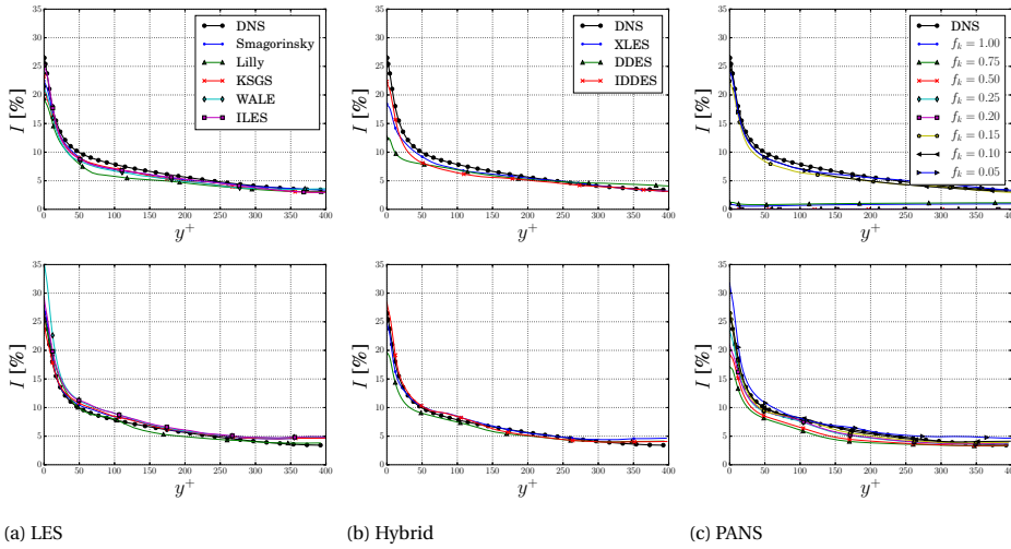
Figure 5.16: Resolved turbulence intensity ( I = 1/3 \sqrt{u'_i u'_i / \bar{u}} ) for recycling (top row) and ITG (bottom row) for LES, hybrid and PANS models. Results obtained at x = 2\delta and averaged in transverse direction.
