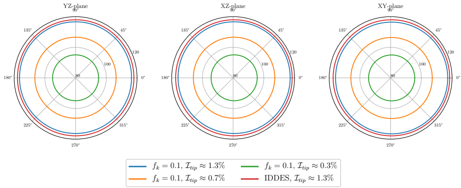
Figure 7.19: OASL for wetted flow computations at receivers in the different planes, integrated over 0.01 \leq 2\pi f r_c / U_\infty \leq 0.1 . For the YZ-plane, 0^\circ is in the lift direction, and 90^\circ in the spanwise direction. For the XZ-plane, 0^\circ is in the flow direction, and 90^\circ in the spanwise direction. For the YZ-plane, 0^\circ is in flow direction, and 90^\circ in the lift direction.
