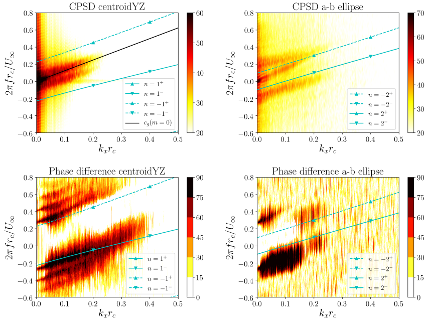
Figure 7.16: PANS ( f_k = 0.1 ), \sigma = 1.7 , \mathcal{J}_{tip} \approx 0.7\% . Wavenumber-frequency diagrams (CPSD) and phase difference of the a-b ellipse and the y-z centroid coordinates, based on FFT with 4 segments in time and 2 in space, with a 75% overlapping Hann window. Phase differences with a coherence below 0.4 are masked. Theoretical dispersion lines shown in cyan, and convection line in black.
