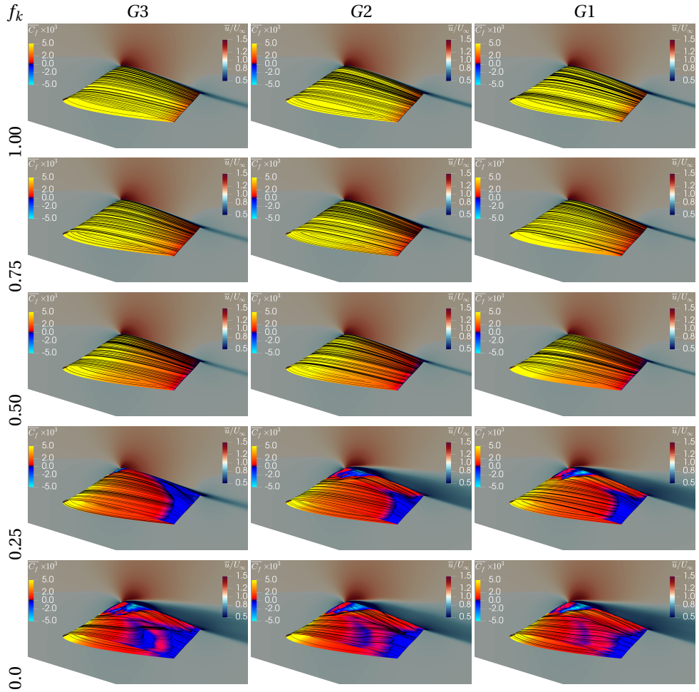
Figure 6.6: Limiting streamlines and time-averaged skin friction coefficient \overline{C_{f,x}} on the wing surface, and streamwise velocity \overline{u}/U_\infty , for different f_k values, using different grids with steady inflow. Results for G4 are similar to G3 and are therefore not shown. Flow from left to right.
