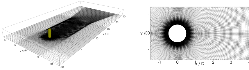
Figure 4.8: Circular cylinder computational domain and grid.
