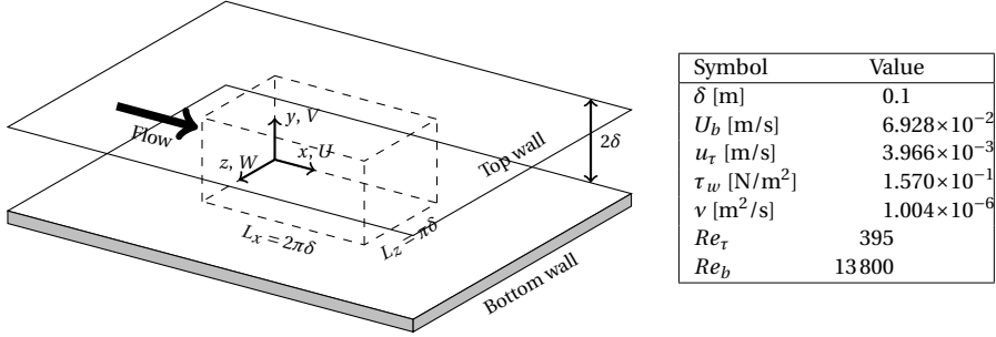
Figure 5.2: Schematic overview of the domain and physical parameters. The dashed lines indicate the computational domain. The figure is based on the drawing of de Villiers [171].
