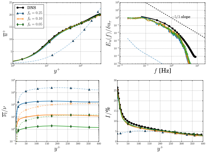
Figure 4.16: Turbulent channel flow. Normalised mean velocity ( \bar{u}^+ = \bar{u}/u_\tau ), turbulence kinetic energy spectra ( E_u(f) at y^+ \approx 20 ), eddy-viscosity ratio ( \nu_t/\nu ) and turbulence intensity ( \mathcal{I} = \bar{u}'_t/U_b ), using PANS-KSKL (solid lines), PANS-SST (dashed lines) and DNS [169]. From left to right, and top to bottom \bar{u}^+ , E_u(f) at y^+ \approx 20 , \nu_t/\nu and \mathcal{I} .
