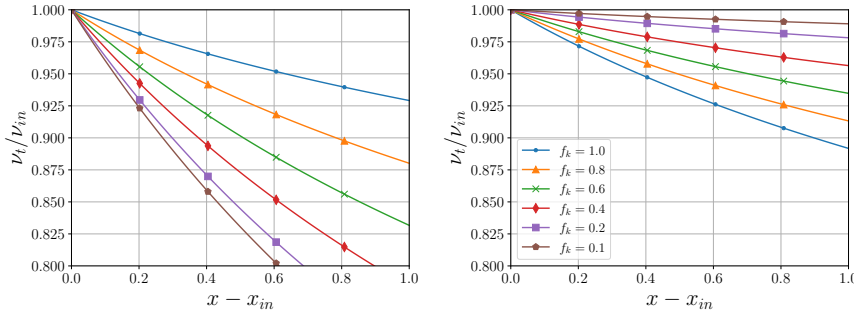
Figure 4.14: Decay of \nu_t versus downstream location x as function of f_k for PANS-SST (left) and PANS-KSKL (right) according to Eq. 4.13 and 4.14, respectively. Values used for this example are C_\mu = 0.09 , \beta^* = 0.09 , \alpha = 0.5 , \zeta_3 = 0.028 , \beta = 0.08 , \langle U \rangle = 1.0 , k_{in}/\nu_{t,in} = 10 .
