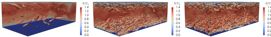
Figure 5.11: Hybrid models instantaneous turbulent flow fields ( Q = 0.3 ), coloured by u^* = u/U_b . From left to right DDES, IDDES and XLES.
