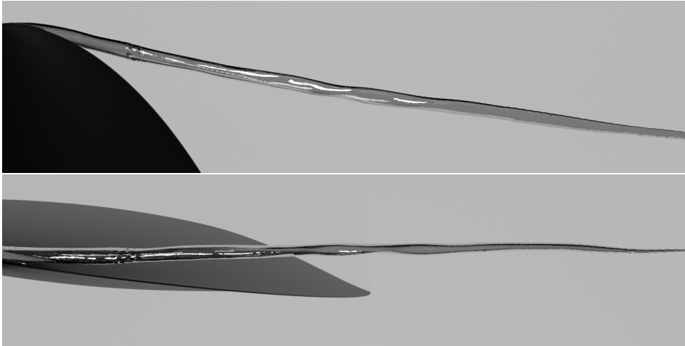
Figure 7.11: PANS ( f_k = 0.1 ), \sigma = 1.7 , \mathcal{J}_{tip} \approx 0.7\% . Instantaneous top and side view images of the vortex cavity. The side view shows the wing pressure side, the flow is from left to right.
