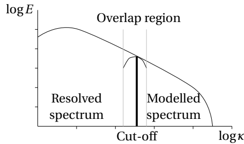
Figure 1.4: Schematic SRS wavenumber energy spectrum, showing the overlap between resolved and modelled velocity scales. E indicates the energy, and \kappa the wavenumber. Based on Reyes et al. [46].
