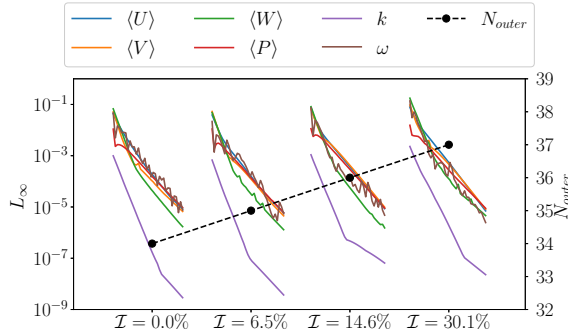
Figure 2.3: Effect of ITG on the L_\infty norm of the residuals of the momentum ( \langle U \rangle , \langle V \rangle and \langle W \rangle ), pressure ( \langle P \rangle ) and turbulence equations ( k and \omega ), for a single timestep. The number of outer loops N_{outer} is also indicated. Results from three simulations with increasing inflow turbulence levels and a reference simulation without resolved inflow turbulence. The residuals are normalised using the diagonal of the matrix on the left-hand side of the linearised system of equations. Figure adapted from Lidtke et al. [127].
