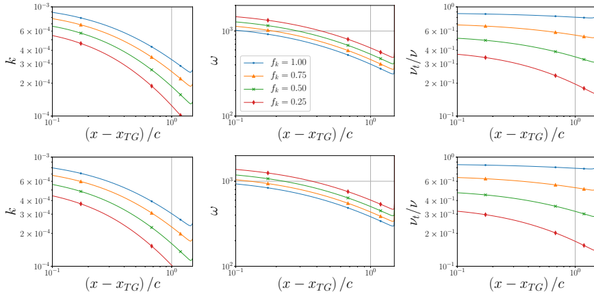
Figure 6.9: Time- and y-z plane spatially-averaged modelled turbulence kinetic energy k (left), dissipation rate \omega (centre) and eddy-viscosity ratio \nu_t/\nu (right) decay for steady inflow. The inlet boundary is located at the left of the figures, the leading edge at the right. Results obtained on grid G4 (top row) and G1 (bottom row) for varying f_k . Recall that for f_k = 0.00 , k and \nu_t/\nu are, by definition, zero.
