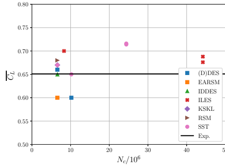
Figure 7.1: Literature overview of lift coefficients ( \overline{C_L} = \overline{L} / (1/2 \rho U_\infty^2 A) ), with the overline indicating a time-average, L the lift force, \rho the density and A the wing surface area) in wetted flow conditions, as function of the number of grid cells ( N_c ) and turbulence model. Results at 9^\circ angle of attack at Re \approx U_\infty c_0 / \nu = 8.95 \times 10^5 . Experimental results from Pennings, Bosschers, et al. [273], numerical results from [25, 190, 202].
