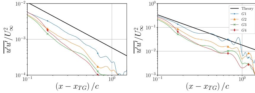
Figure 6.11: Time- and y - z plane spatially-averaged resolved streamwise Reynolds stresses for Case A (left) and B (right) between ITG and the leading edge, on different grids for f_k = 0.25 . The results show little dependence on f_k .
