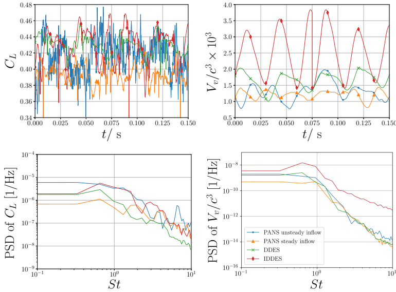
Figure 6.21: Time signal and PSD with windowing of lift coefficient (left) and vapour volume (right), for f_k = 0.25 on grid G1 without and with inflow turbulence ( \mathcal{L}/c = 0.013 , \mathcal{J}_{LE} = 6.3\% ). Time axis shifted following removal of start-up effects. DDES results from Vaz et al. [79].
