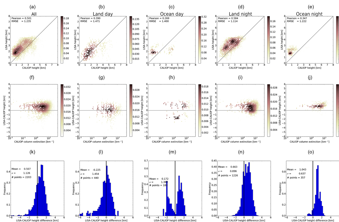
Figure A8. Similar to Fig. A5 but for the LISA algorithm.
