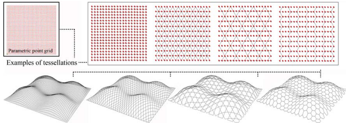
Fig. 3: Examples of tessellations based on the point grid.
