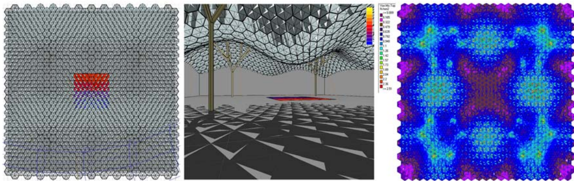
Fig 6: examples from current analysis: left: solar energy; right: structural behaviour
