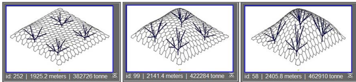
Fig 4: examples of instances from the first testing analysis (structural behaviour)
