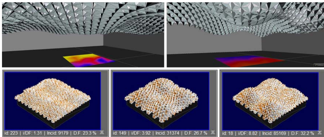
Fig 5: second testing analysis (solar energy). Top Left: example with north facing opaque panels. Top Right, Bottom: examples with south facing opaque panels.
