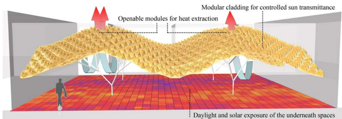
Fig. 1: Concept of SolSt.
