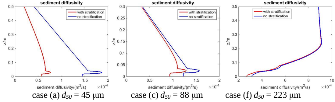
Fig. 20. Comparison of the calculated sediment diffusivity profiles with and without stratification effects
