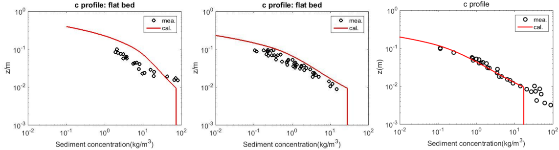
Fig. 8. Verification of the experimental data of Dohmen Janssen et al. (2001) ( u_c is current velocity)
