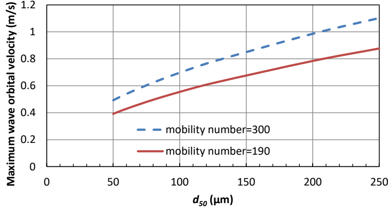
Fig. 3. The criterion conditions of bed forms according to d_{50} and the maximum wave orbital velocity u_m (extrapolated by O'Donoghue et al. (2006)'s criterion)
