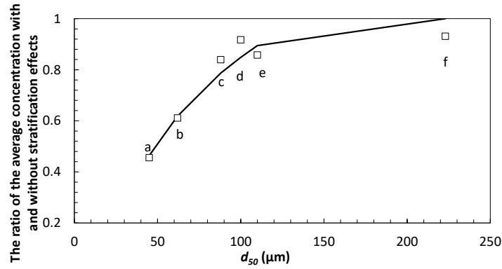
Fig. 21. The ratio of the average sediment concentration with and without stratification effects of the study cases
