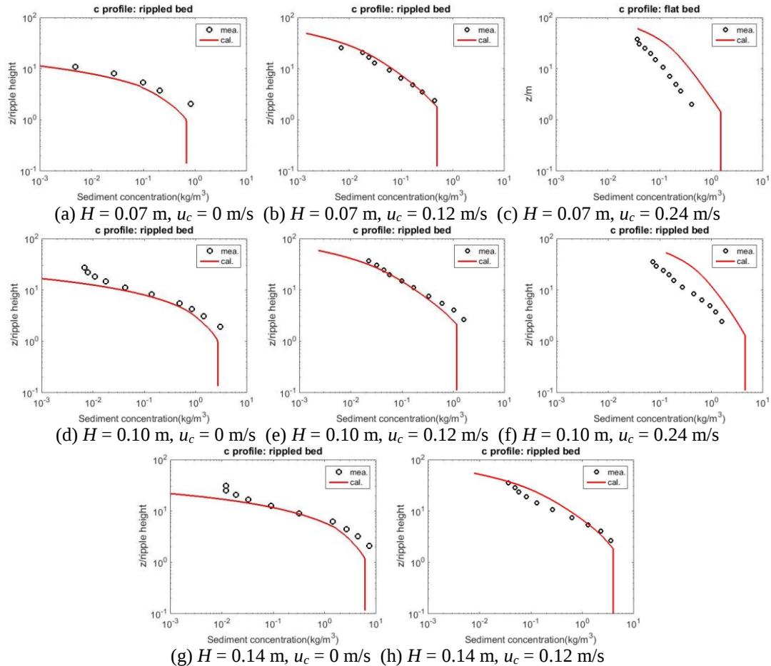
Fig. 12. Verification of the experimental data of Havinga (1992) ( H is wave height, h = 0.4 m, d_{50} = 100 \mu\text{m} )
