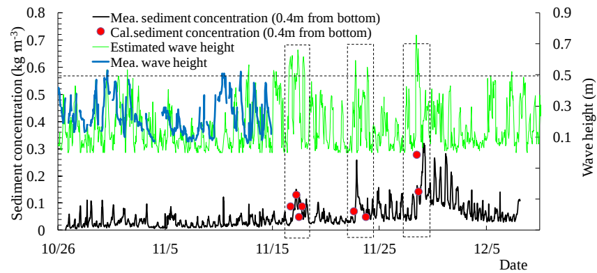
Fig. 10. Comparison of the calculated and measured concentration in Caofeidian sea area
