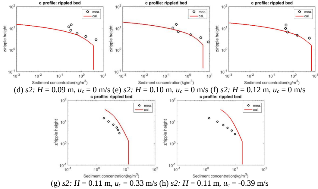
Fig. 16. Verification of the experimental data of Yao et al. (2015) ( h = 0.3 m, T = 1.5 s, s1: d_{50} = 44 \mu m, s2: d_{50} = 88 \mu m)
