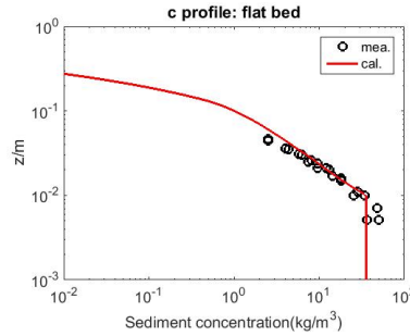
Fig. 7. Verification of the experimental data of Ribberink and Al-Salem (1995)
