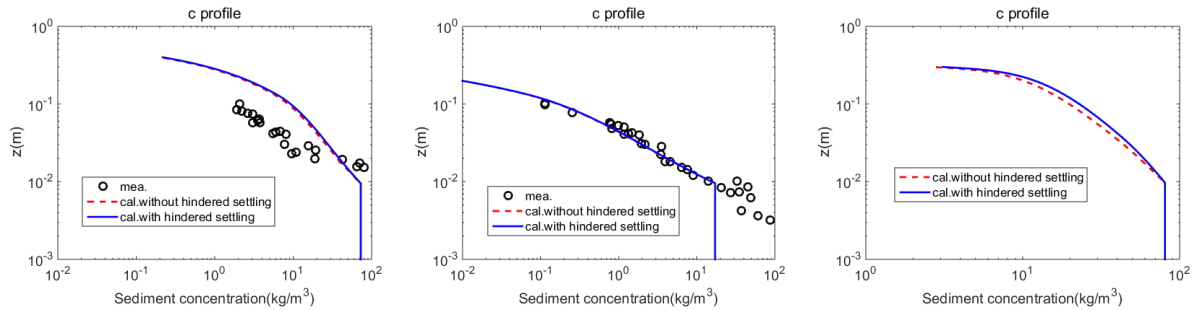
Fig. 22 Comparison of sediment concentration with and without hindered settling velocity ((a) Dohmen Janssen et al. (2001), d_{50} = 0.13 mm, u_c = 0.24 m/s; (b) Dohmen Janssen et al. (2001), d_{50} = 0.32 mm, u_c = 0.26 m/s; (c) d_{50} = 0.062 mm, u_m = 1.0 m/s, u_c = 0.6 m/s, h = 0.3 \text{ m} )
