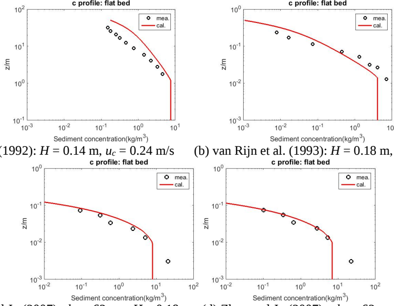
Fig. 17. Verification of the experimental data of Havinga (1992), van Rijn et al. (1993) and Zhou and Ju (2007)
