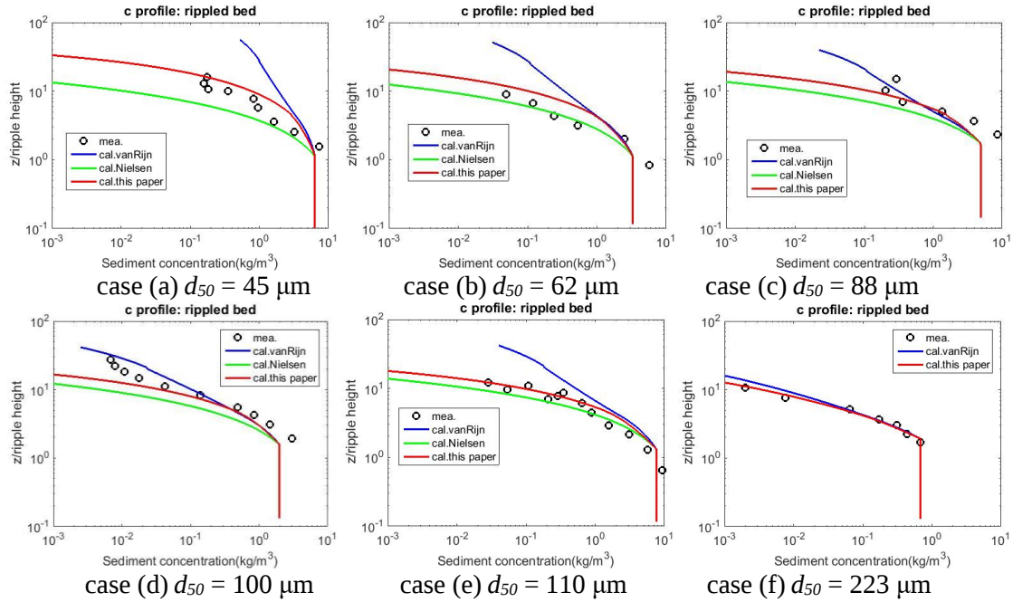
Fig. 18. Comparison of sediment concentration profile by different formulas (case (a): based on Li (2014)'s experiment with H = 0.18 m; case (b): based on Zhou and Ju (2007)'s experiment with H = 0.12 m; case (c): based on Yao et al. (2015)'s experiment with H = 0.10 m; case (d): based on Havinga (1992)'s experiment with H = 0.10 m; case (e): based on Li (2014)'s experiment with H = 0.18 m; case (f): based on van Rijn et al. (1993)'s experiment with H = 0.15 m and u_c = 0.13 m/s)
