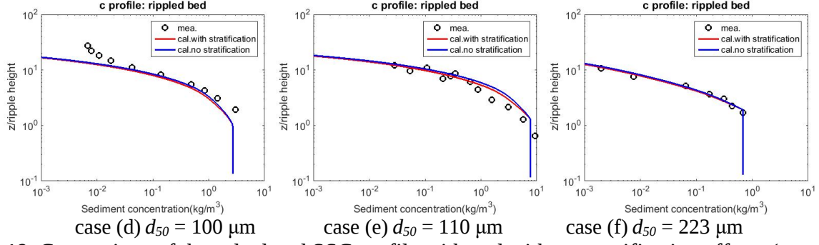
Fig. 19. Comparison of the calculated SSC profile with and without stratification effects (case (a): based on Li (2014)'s experiment with H = 0.18 m; case (b): based on Zhou and Ju (2007)'s experiment with H = 0.12 m; case (c): based on Yao et al. (2015)'s experiment with H = 0.10 m; case (d): based on Havinga (1992)'s experiment with H = 0.10 m; case (e): based on Li (2014)'s experiment with H = 0.18 m; case (f): based on van Rijn (1993)'s experiment with H = 0.15 m and u_c = 0.13 m/s)
