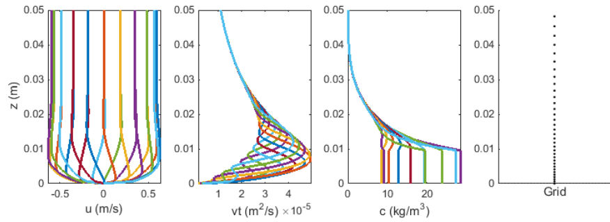
Fig. 2. Intra-wave process of velocity profiles (left column), eddy viscosity profiles (middle column) and sediment concentration profiles (right column) in plane bed conditions calculated by the 1DV model (The calculation conditions: h = 0.3 m, u_m = 0.6 m/s, T = 3 s and d_{50} = 0.062 mm)
