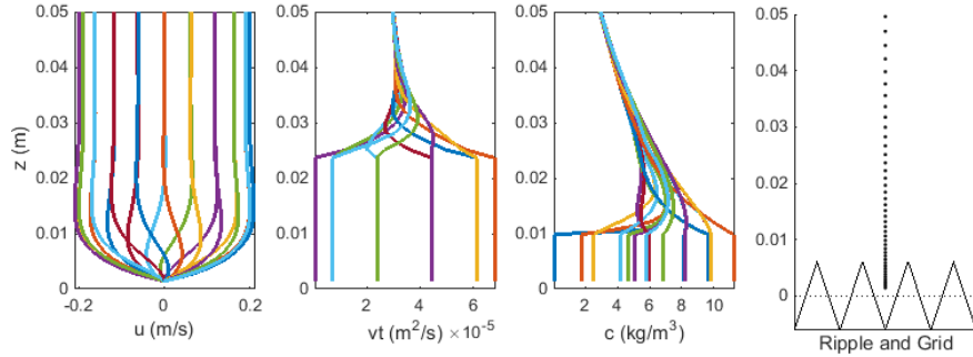
Fig. 1. Intra-wave process of velocity profiles (left column), eddy viscosity profiles (middle column) and sediment concentration profiles (right column) over rippled bed calculated by the 1DV model (The calculation conditions: water depth h=0.3 m, maximum wave orbital velocity u_m = 0.2 m/s, wave period T = 3 s and d_{50} = 0.062 mm)
