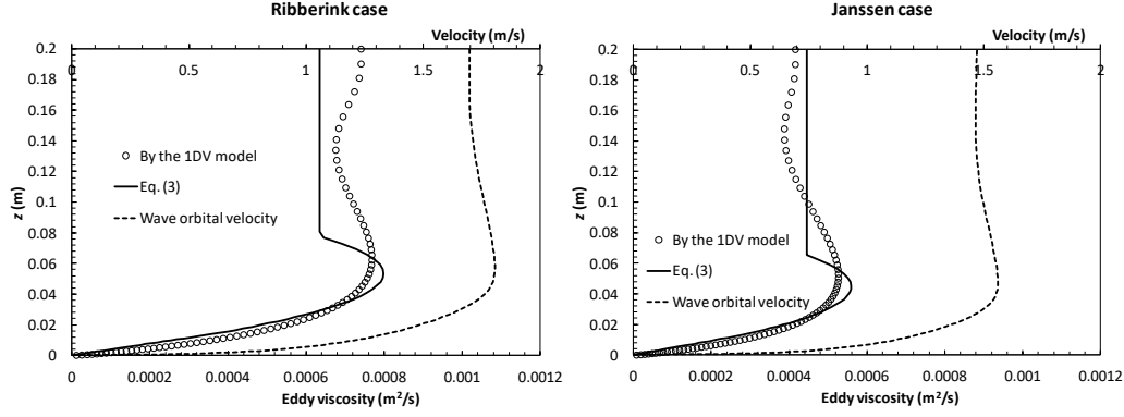
Fig. 4. Comparison of the calculated mean eddy viscosity distribution with the results of the 1DV model (the wave conditions were after Dohmen Janssen et al. (2001) and Ribberink and Al-Salem (1995))
