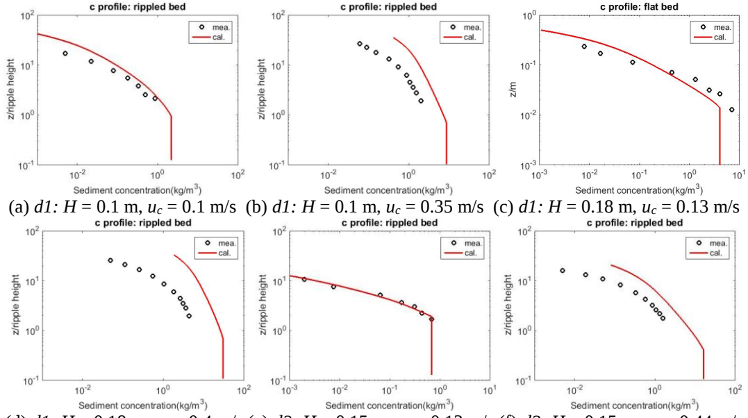
Fig. 13. Verification of the experimental data of van Rijn et al. (1993) ( h = 0.4 m, d1 : d_{50} = 110 \mu\text{m} and d2 : d_{50} = 200\text{--}220 \mu\text{m} )
